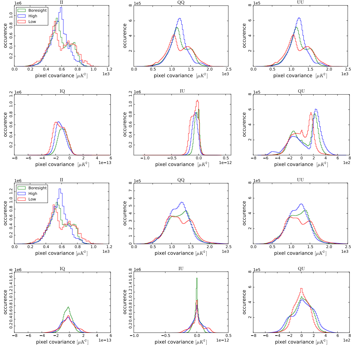
Figure 4. Histograms of the 3 \times 3 pixel covariance matrix elements in Ecliptic coordinates (first and second rows) and in Galactic coordinates (third and fourth rows). There are minimal intensity-to-polarization couplings (notice the change of scale) but significant QU residual correlation.
