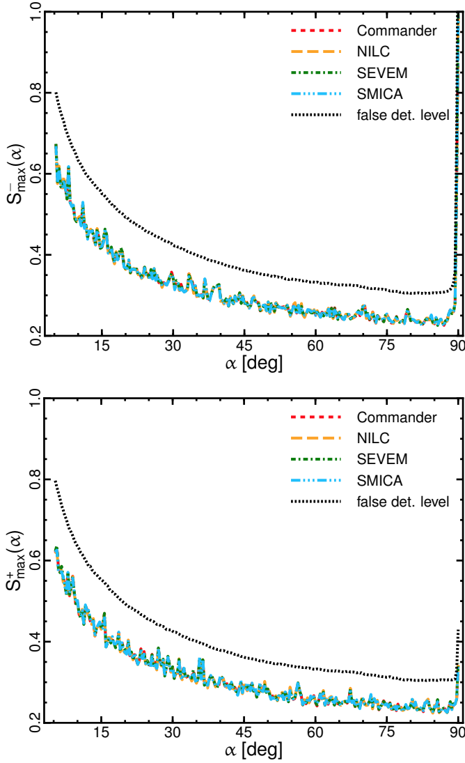
Fig. 11. S_{\max}^{-} (upper) and S_{\max}^{+} (lower) statistics as a function of circle radius \alpha for the Planck Commander (short-dashed red line), NILC (long dashed orange line), SEVEM (dot-dashed green line), and SMICA (three dot-dashed blue line) 2015 temperature maps. The dotted line shows the false detection level established such that fewer than 1% of 300 Monte Carlo simulations of the SMICA CMB temperature map, smoothed and masked in the same way as the data, would yield a false event. The peak at 90^\circ corresponds to a match between two copies of the same circle of radius 90^\circ centred around two antipodal points.
