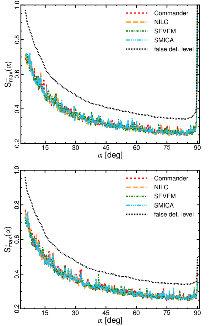
Fig. 12. S_{\max}^{-} (upper) and S_{\max}^{+} (lower) statistics as a function of circle radius \alpha for the Planck Commander (short-dashed red line), NILC (long dashed orange line), SEVEM (dot-dashed green line), and SMICA (three dot-dashed blue line) E -mode maps. The dotted line shows the false detection level established such that fewer than 1% of 300 Monte Carlo simulations of the SMICA CMB E -mode map, smoothed and masked in the same way as the data, would yield a false event. The peak at 90^\circ corresponds to a match between two copies of the same circle of radius 90^\circ centred around two antipodal points.
