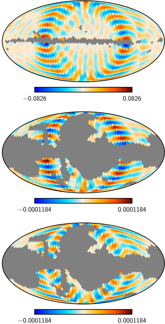
Fig. 5. Mode structure plotted as maps for the eigenvector corresponding to the 301st-highest-signal eigenvalue of the fiducial simply-connected model. The top map corresponds to temperature, middle to Q polarization, and bottom to U polarization. Masked pixels are plotted in grey.
