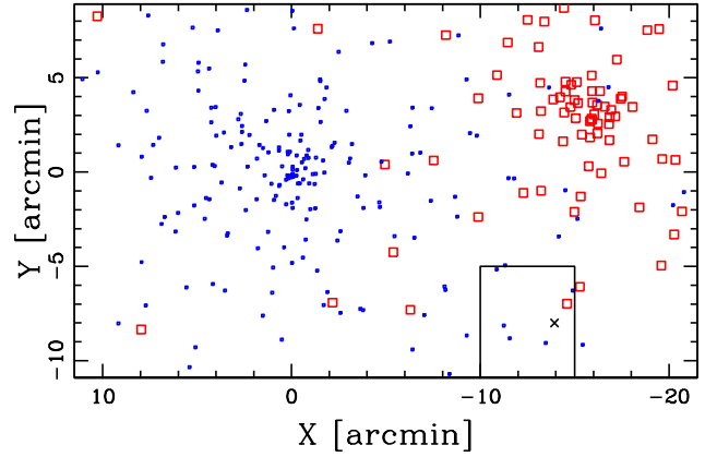
Fig. 10. Spatial distribution of simulated galaxies of RXCJ1825 + CIZAJ1824 system. Blue and red points indicate galaxy points of RXCJ1825 and CIZAJ1824, at low and high velocities, respectively. The black cross indicates the position of SG and the rectangle delimits a region close to SG where the real velocity field is characterized by high velocities (cf. Figs. 7 and 8, lower panel).
