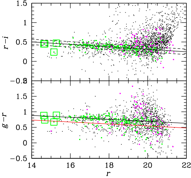
Fig. 5. Upper panel: Pan-STARRS r-i vs. r diagram. Small black symbols indicate the galaxies of the photometric catalog, green and magenta symbols indicate member and non-member galaxies of our spectroscopic catalog, large green squares indicate prominent galaxies (BCG-E, BCG-CC, BCG-W, and SG in order of increasing r magnitude). The solid line gives the CMR determined on spectroscopic member galaxies; the dashed lines are drawn at \pm 0.07 mag from this value and are used to define the photometric members in the Pan-STARRS catalog. Lower panel: same as above, but for Pan-STARRS g-r vs. r diagram. The red solid is drawn at 0.15 mag down to the CMR and is used to discriminate red from blue galaxies.
