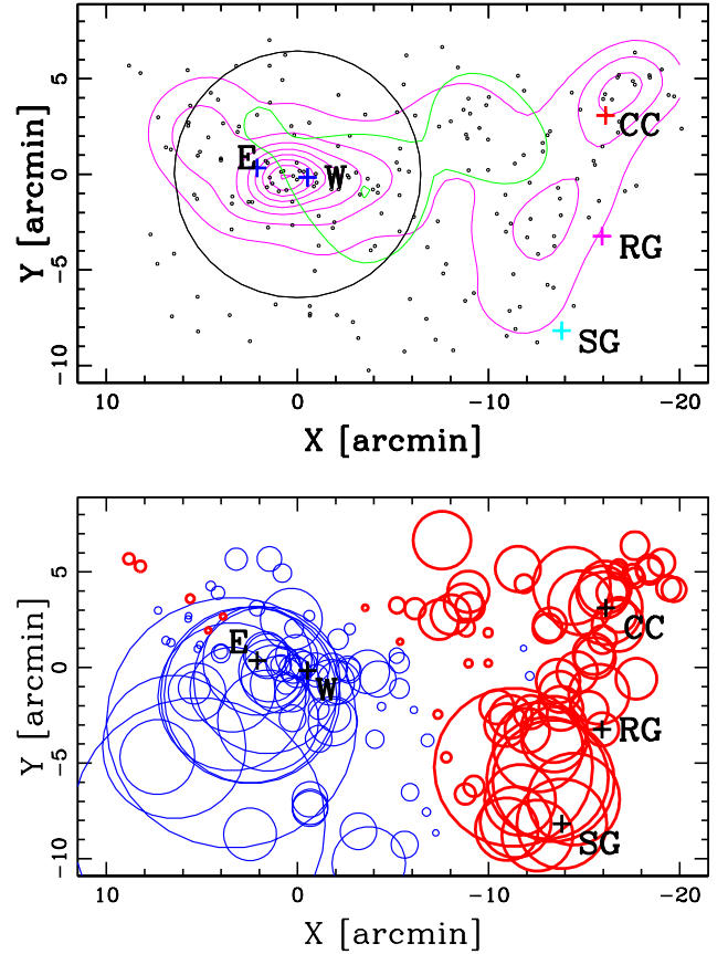
Fig. 8. Upper panel: same as Fig. 4, but with isodensity contours for 41 blue galaxies (in green) and 153 red galaxies (in magenta). Lower panel: same as Fig. 7, but for 153 red galaxies.
