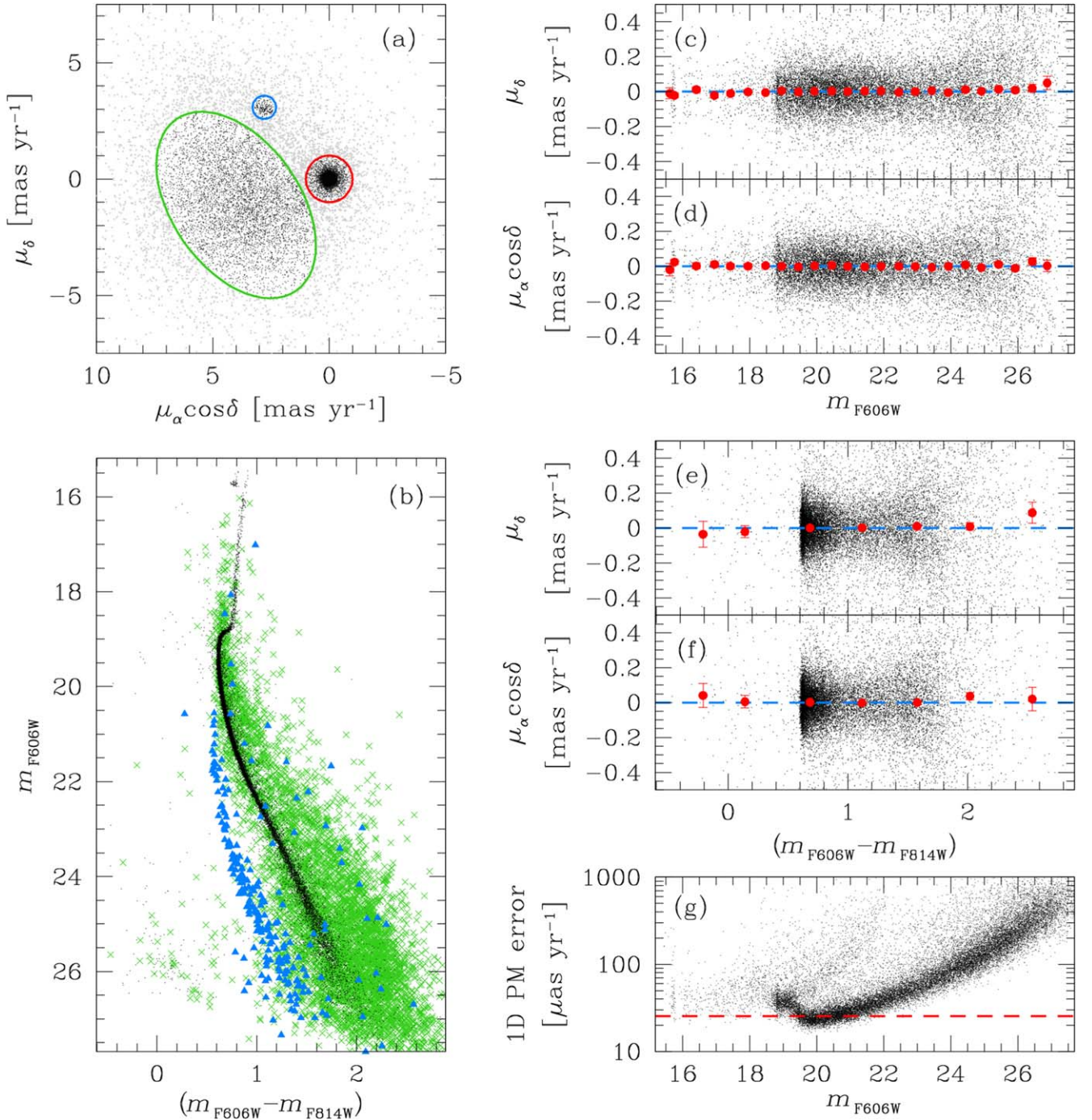
Figure 3. Overview of the PM catalog of NGC 6652. (a) The VPDs of the relative corrected PMs. The stars within the red circle (centered on the origin of the VPD and with radius of 1 mas yr -1 ) are likely cluster members, while the blue circle marks the location of Sagittarius Dwarf objects, and with the green ellipse highlighting a group of Bulge stars. The gray dots are all sources outside any of these three selections (likely Bulge objects or cluster stars with large PM uncertainties). (b) The m_{F606W} vs. (m_{F606W} - m_{F814W}) CMD. The black dots are likely cluster members; the blue triangles are members of the Sagittarius Dwarf; and the green crosses are Bulge objects (the gray points in the VPD are not shown for clarity). (c) and (d) \mu_\delta and \mu_\alpha \cos \delta PMs as a function of m_{F606W} . Only members of NGC 6652 are shown (the black points). The red points (with error bars) are the median values of the PMs in 0.5 mag bins. The azure line is set to zero. (e) and (f): \mu_\delta and \mu_\alpha \cos \delta PMs as a function of (m_{F606W} - m_{F814W}) . Panels (c) to (f) show no obvious trends of our corrected PMs with stellar magnitude or color. (g) 1D corrected PM error (the sum in quadrature of the PM errors in each direction, divided by \sqrt{2} ) as a function of m_{F606W} . The red line is set at the median value of the 1D PM errors of bright, well-measured unsaturated stars.
