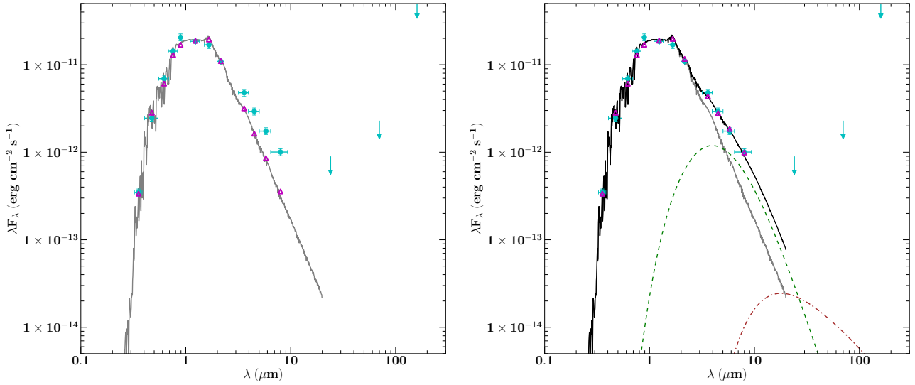
Fig. 1. Spectral energy distribution of CoRoT 223992193 (cyan points) with upper limits in the far-infrared (cyan arrows). This figure is identical to Fig. 13 of Gillen et al. (2014, Paper I); it is reproduced here for clarity. Left: the grey line and magenta triangles show the best-fit model using two naked photospheres. Right: the black line and magenta triangles show the best-fit two naked photospheres model with a small amount of hot dust in the inner cavity of the circumbinary disk. The stellar and hot dust terms are shown separately as the grey solid and dashed green lines, respectively. Also shown for completeness, but not used in the fit, is the expected emission from a razor-thin circumbinary disk extending down to 22 R_{\odot} (brown dot-dashed line), which is illuminated by the central star and heated by the gravitational potential energy released from accretion with \dot{M} = 10^{-11} M_{\odot} \text{ yr}^{-1} .
