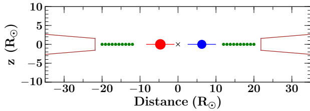
Fig. 2. Schematic representation of the proposed system geometry, showing distance from the centre of mass against height above the system plane ( z ). This figure is identical to Fig. 14 of Gillen et al. (2014, Paper I); it is reproduced here for clarity. The primary and secondary stars, along with their circumstellar disks (truncated to a third of the binary separation), are shown in red and blue respectively (the circumstellar disks are shown for completeness but there is no direct evidence for their presence). The sizes and separations of the two stars are to scale. The circumbinary disk (brown) has its inner radius truncated at twice the binary separation. The green dots indicate the general location of dust lying within the inner cavity of the circumbinary disk, such as one could expect to find in accretions streams.
