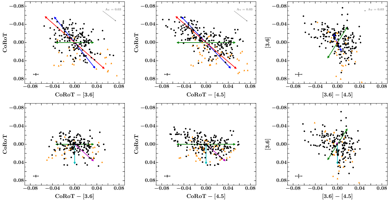
Fig. 9. Colour–magnitude diagrams. Top row, left to right: raw light curve data (black points) in the CoRoT vs. CoRoT–[3.6], CoRoT vs. CoRoT–[4.5] and [3.6] vs. [3.6]–[4.5] spaces. Data masked in the spot modelling are shown by the orange triangles. Coloured arrows show the effects of different types of variability: cold spots (blue), hot spots (red) and dust emission (green). Grey arrows indicate the direction of interstellar dust extinction. Bottom row, left to right: same as for the top row but showing the residuals of the spot modelling. Magenta and cyan arrows indicate the effects of obscuration by small and large dust grains, respectively. The error bar in the bottom left corner of each subplot shows a representative uncertainty for each data point. All plots share common axes.
