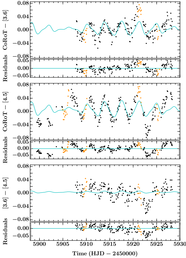
Fig. 8. CoRoT and Spitzer colour vs. time relations. Top to bottom: CoRoT-[3.6], CoRoT-[4.5] and [3.6]-[4.5], with residuals immediately below in each case. Black points show data used in the spot modelling, orange points indicate data that was masked in the fit and the cyan line represents the colour signature of the spot model. All colour-time relations display quasi-sinusoidal variations, which can most clearly be seen comparing the widely separated bandpasses of the CoRoT-[4.5] colour space. All plots share common axes.
