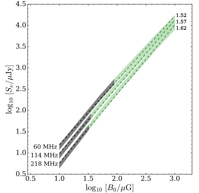
Fig. 4. Flux density at 60, 114, and 218 MHz (lower-left labels) as a function of magnetic field strength B_0 for model B (see Sect. 5.1). Green shaded areas encompass the curves obtained with Eq. (9) by using \kappa = 0.5 and 0.7. Grey areas correspond to S/N < 3 and dashed lines are power-law fits of S_\nu \propto B_0^\delta with \delta listed in the upper-right corner.
