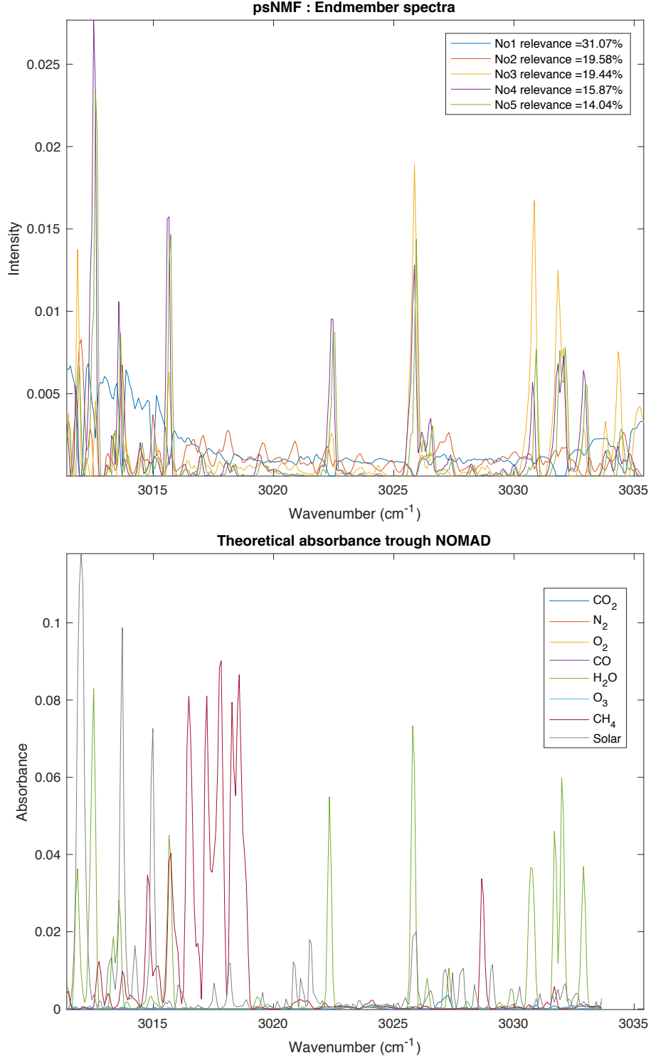
Figure 9: Results of the psNMF algorithm for the diffraction order 134 for N_S = 5 . The source 1 is identified to the background level (continuum misestimation), the sources 3, 4 and 5 are identified to \text{H}_2\text{O} . The sources 2 present unmodeled lines that are not present in the spectroscopic database. These lines has been first detected in the ACS instrument data and attributed to \text{CO}_2 magnetic dipole transition (Trokhimovskiy et al., 2020). No source seems to be related to \text{CH}_4 .
