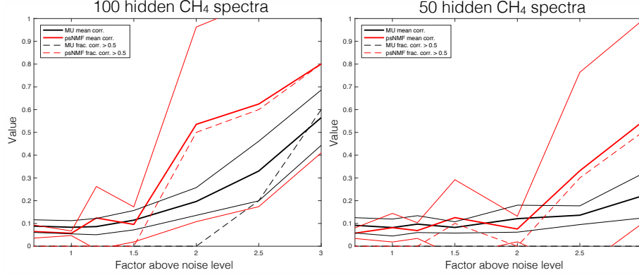
Figure 6: Results of the MU and psNMF algorithm for N_S = 5 , N_O = 10000 , N_\nu = 320 , as a function of the factor above noise level. The average Q of 10 realizations of the best estimated source (thick lines and standard deviation in thin lines) and the fraction of acceptable results (with Q > 0.5 ). (left) with 100 hidden \text{CH}_4 spectra (right) with 50 hidden \text{CH}_4 spectra
