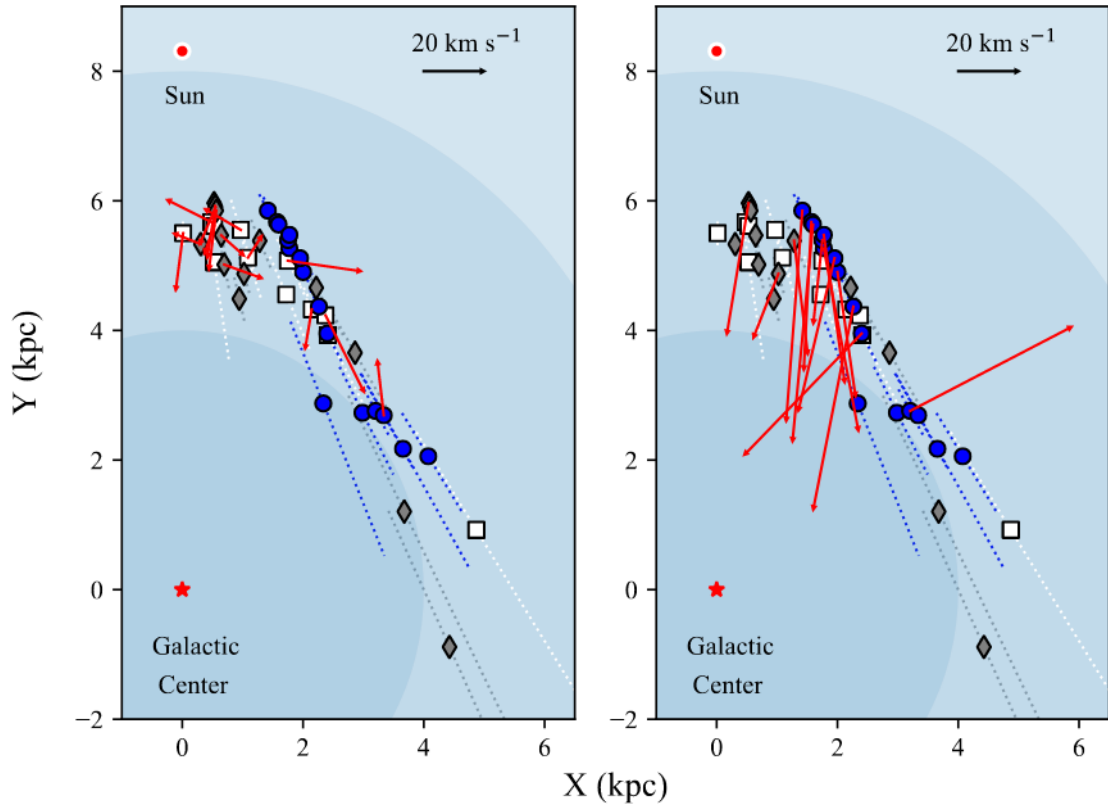
Figure 3: Same as Fig. 2a but with peculiar motion vectors overlayed (left: peculiar motion \leq 20 \text{ km s}^{-1} , right: peculiar motion > 20 \text{ km s}^{-1} ). The vectors have uncertainties of < 20 \text{ km s}^{-1} . Distance uncertainties are shown as dashed lines.
