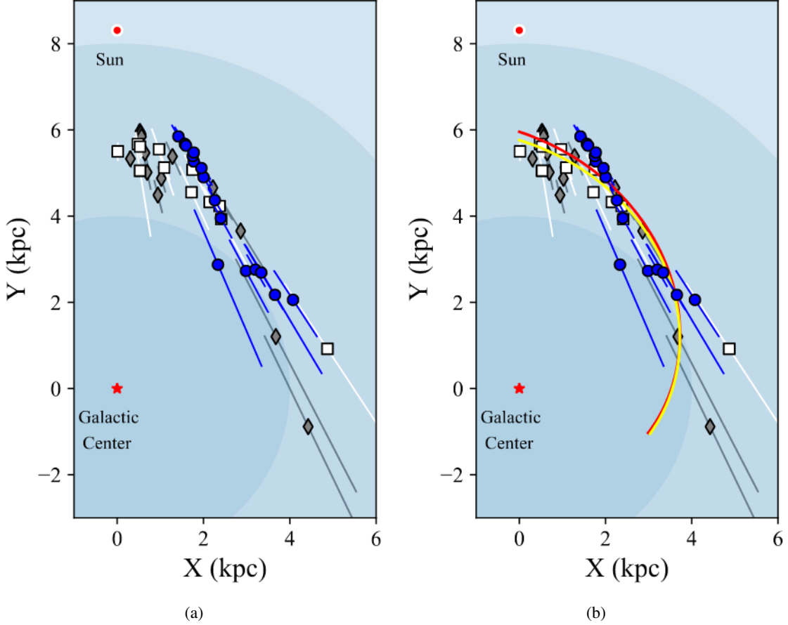
Figure 2: Left panel: XY plot of the 43 masers in the Scutum spiral arm (grey diamonds: published sources in Sato et al. (2014), blue circles: sources in Immer et al. (2019, subm.), white squares: sources in Li et al. (2019, in prep.)). The position of the Sun and the Galactic Center are marked. Distance uncertainties are shown as continuous lines. Right panel: As left panel, but with two pitch angle fits overlayed (yellow: Sato et al. (2014), red: Li et al. (2019, in prep.)).
