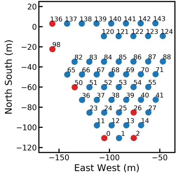
Figure 4. HERA 52 antenna configuration. Malfunctioning elements highlighted in red for 2018 December 24, 25, and 26 were not included in this work.
