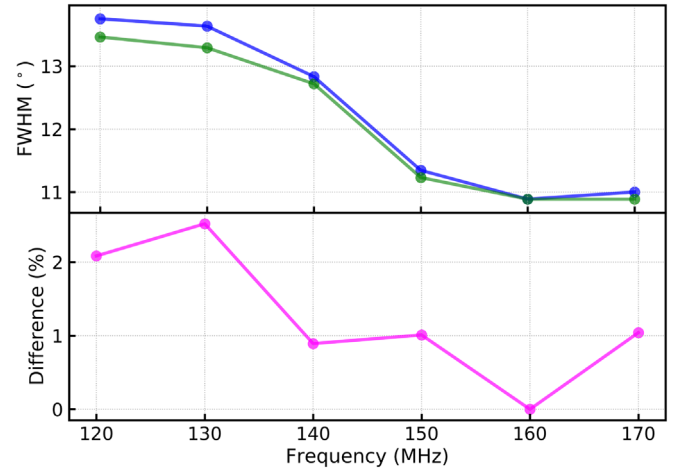
Figure 19. Top: FWHM evaluated using the beam solutions along the east–west polarization illustrated in Figure 15 (blue) and EM simulations (green) at various frequencies. Bottom: the percentage difference in FWHM relative to the EM simulations. We observe a good agreement between the beam solutions and EM simulations.
