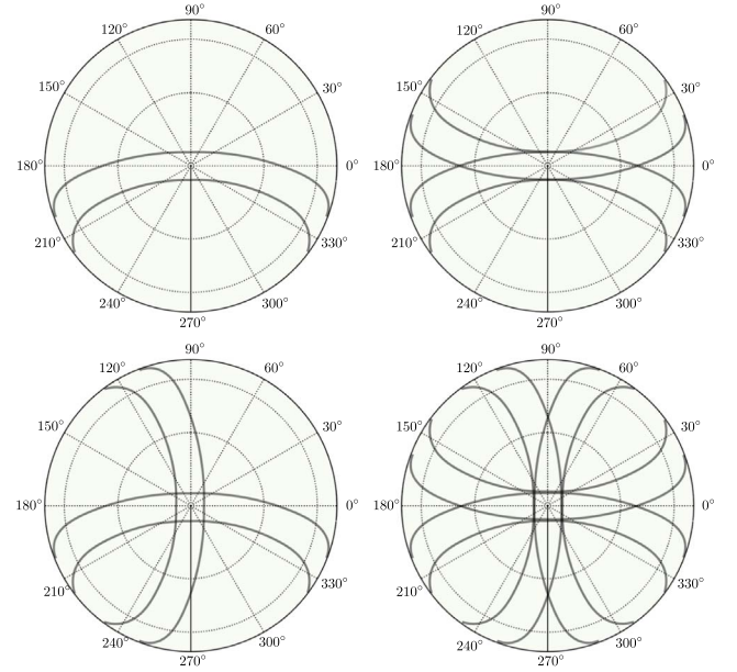
Figure 1. Top left: a schematic representation of two arbitrary source tracks crossing the primary beam of our instrument. Top right: source tracks overlaid with the corresponding 180^\circ mirrored tracks. Bottom left: source tracks overlaid with the corresponding 90^\circ rotated tracks. Bottom right: source tracks overlaid with a combination of 180^\circ mirrored tracks, and 90^\circ and 270^\circ rotated tracks. The projection is orthographic with the center indicating zenith and the dotted lines are spaced 30^\circ .
