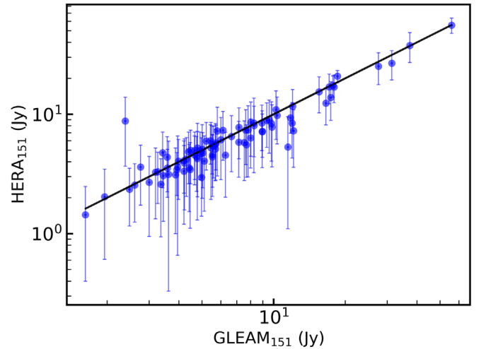
Figure 20. Flux densities of the 90 matching components from GLEAM S_{G151} plotted against the derived flux densities S_{151} reported in Table 2. Most of our flux measurements align with the GLEAM results within the quoted errors except a few, namely “J061721–282547,” “J094953–251138,” and “J103312–341842.”
