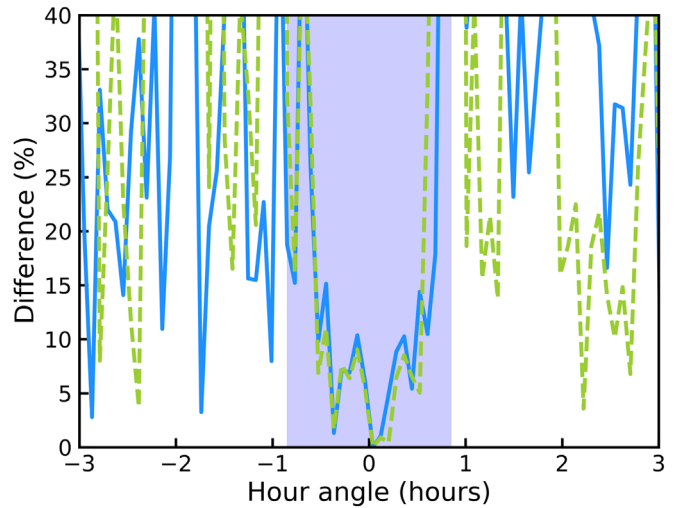
Figure 22. Simulations demonstrating that confusion noise is the dominant systematics in our approach. Adding Gaussian noise to our simulations yields negligible change inside the main lobe. We plot the percentage difference between the input and recovered beam of a transiting arbitrary source evaluated from a noiseless simulation, in blue. We added Gaussian noise to the simulations, and the resulting difference is plotted in green. The shaded area represents the main lobe of the beam response.
