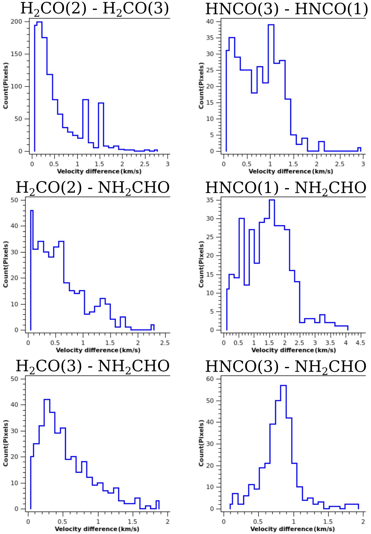
Fig. C.3. G24A2(N) first moment difference histogram.
