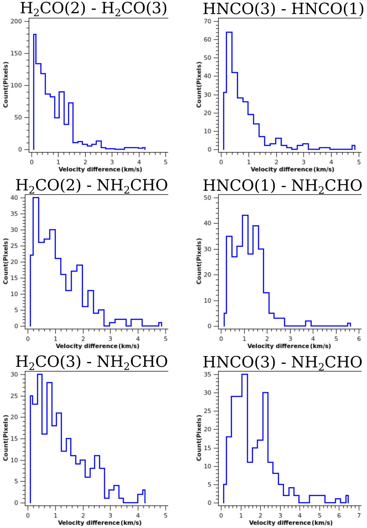
Fig. C.4. G24A2(S) first moment difference histogram.
