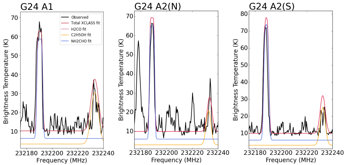
Fig. 2. Observed and synthetic spectra of G24 A1 (left), A2(N) (middle), and A2(S) (right) with fits showing NH 2 CHO (2) (dark blue). The continuum levels are offset for easy viewing.
