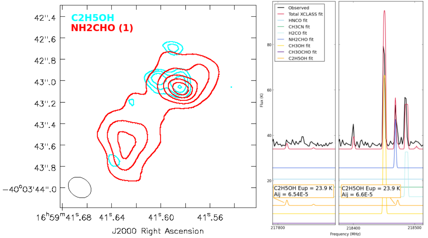
Fig. A.1. Right: spectrum of G345 NW spur showing a \text{C}_2\text{H}_5\text{OH} transition ( 5_{3,3}-4_{2,2} ) at 217 803 MHz with the same E_{\text{up}} and nearly equal A_{ij} as the \text{C}_2\text{H}_5\text{OH} transition ( 5_{3,2}-4_{2,3} ) that is blended with the \text{NH}_2\text{CHO} (1) transition (at 218 461 MHz). Left: contours of the integrated intensity map of this \text{C}_2\text{H}_5\text{OH} line is overlaid on the map of the \text{NH}_2\text{CHO} (1) transition to show that the strength and spatial extent is different.
