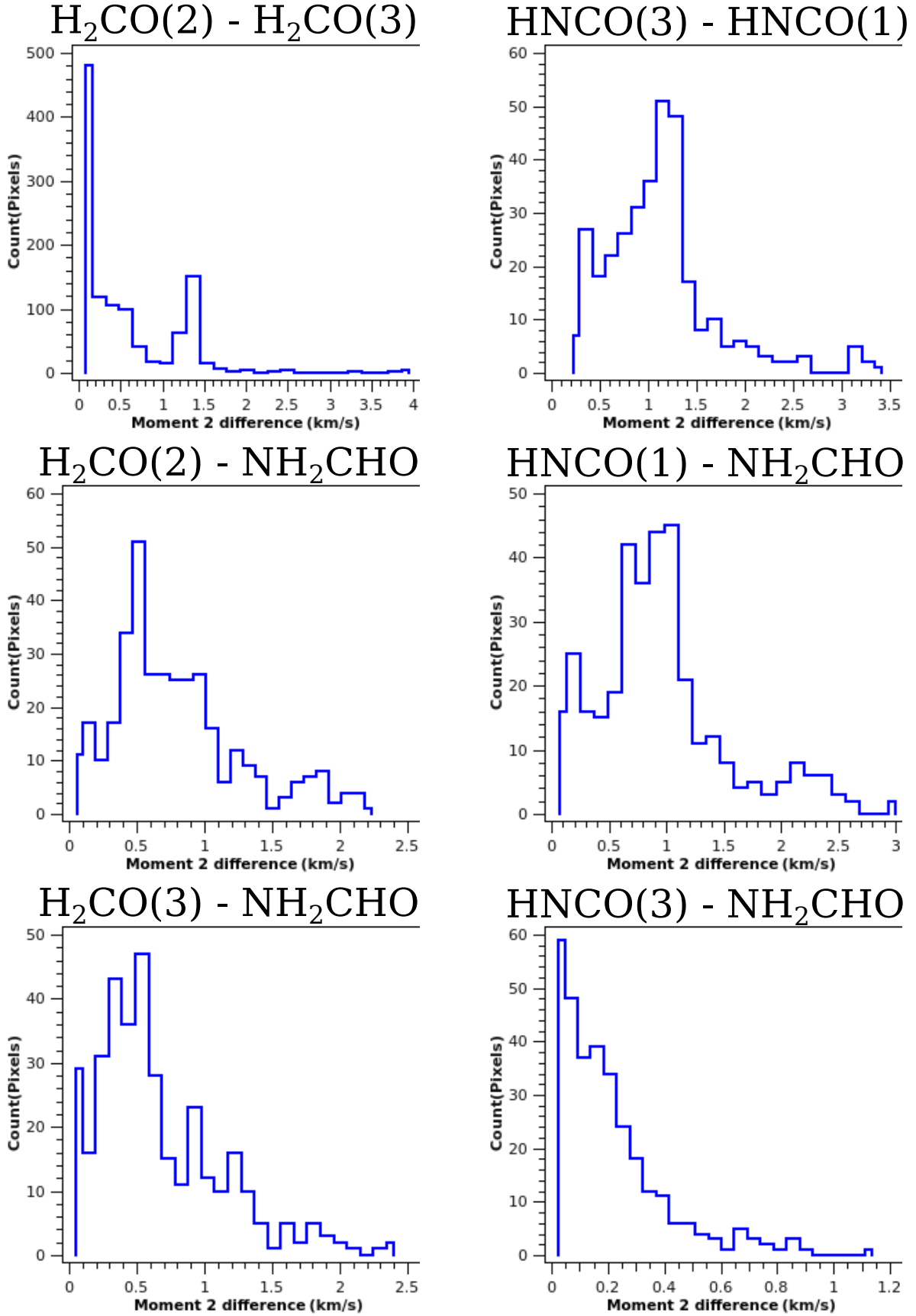
Fig. C.9. G24A2(N) second moment difference histogram.
