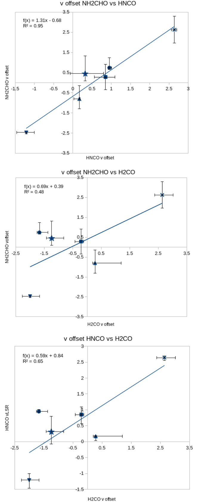
Fig. 17. XCLASS determined velocity offset comparison between NH 2 CHO and HNCO ( top ), NH 2 CHO and H 2 CO ( middle ), and HNCO and H 2 CO ( bottom ). The symbols are as in Fig. 16.
