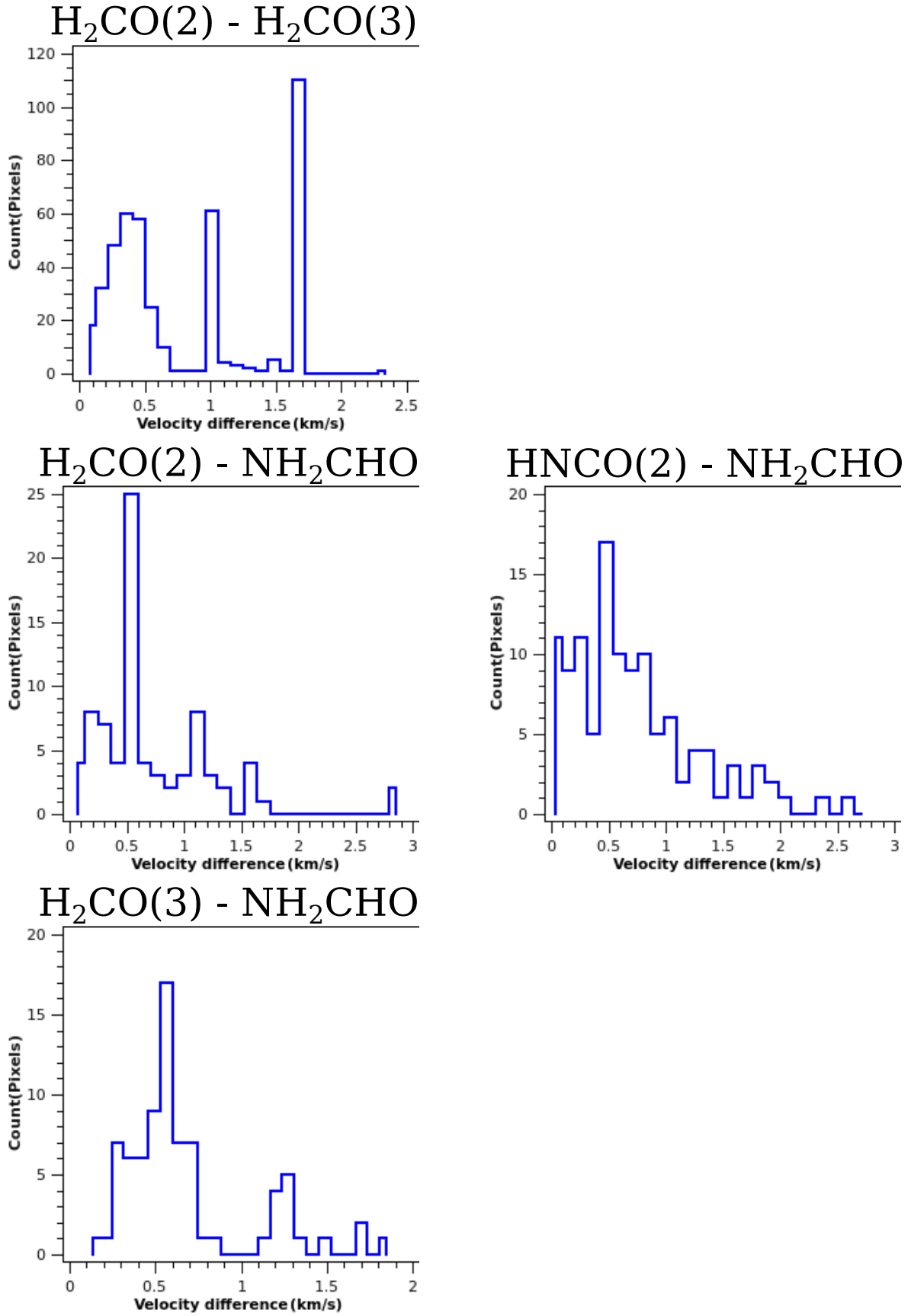
Fig. C.1. G17 first moment difference histogram.
