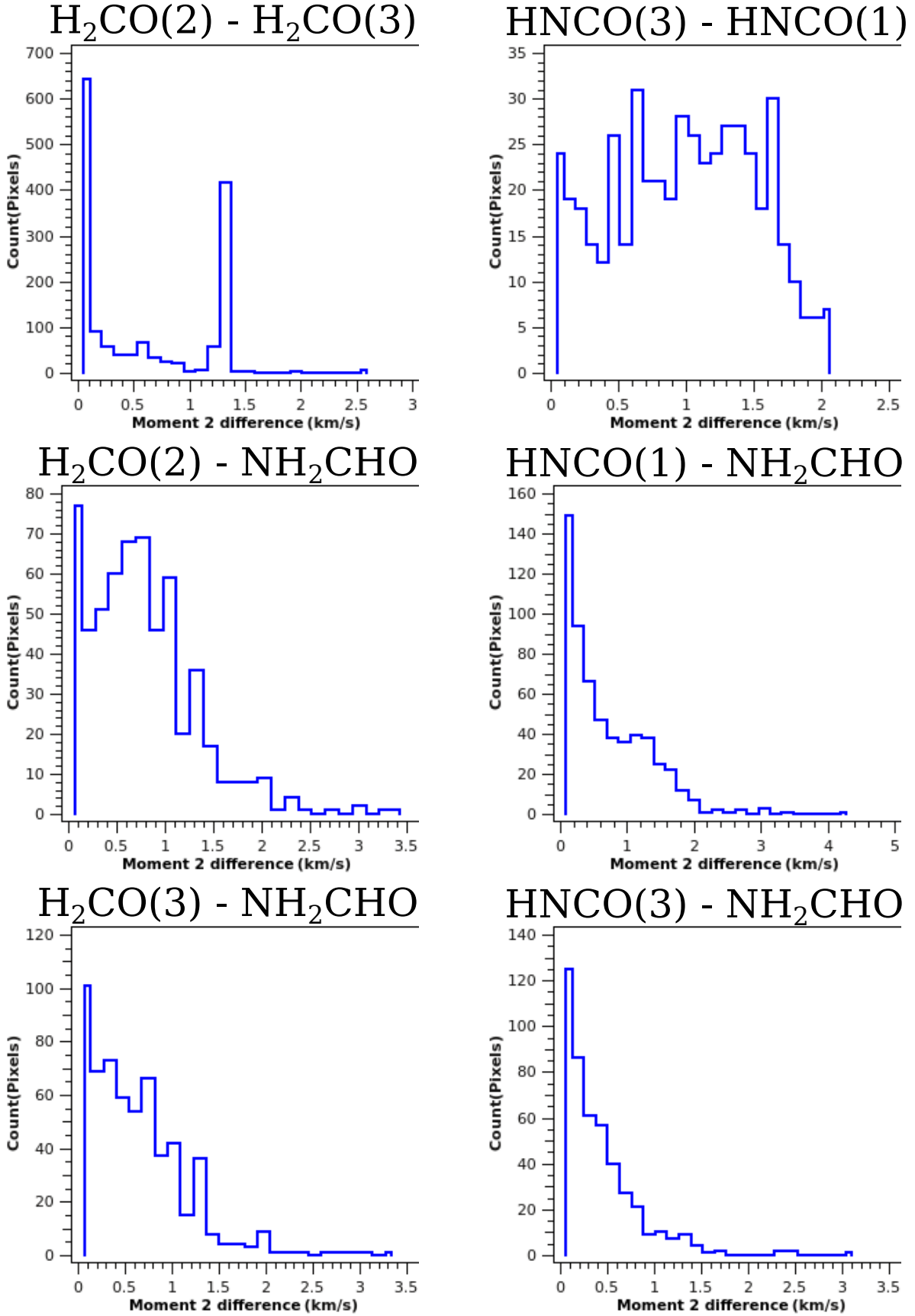
Fig. C.8. G24A1 second moment difference histogram.
