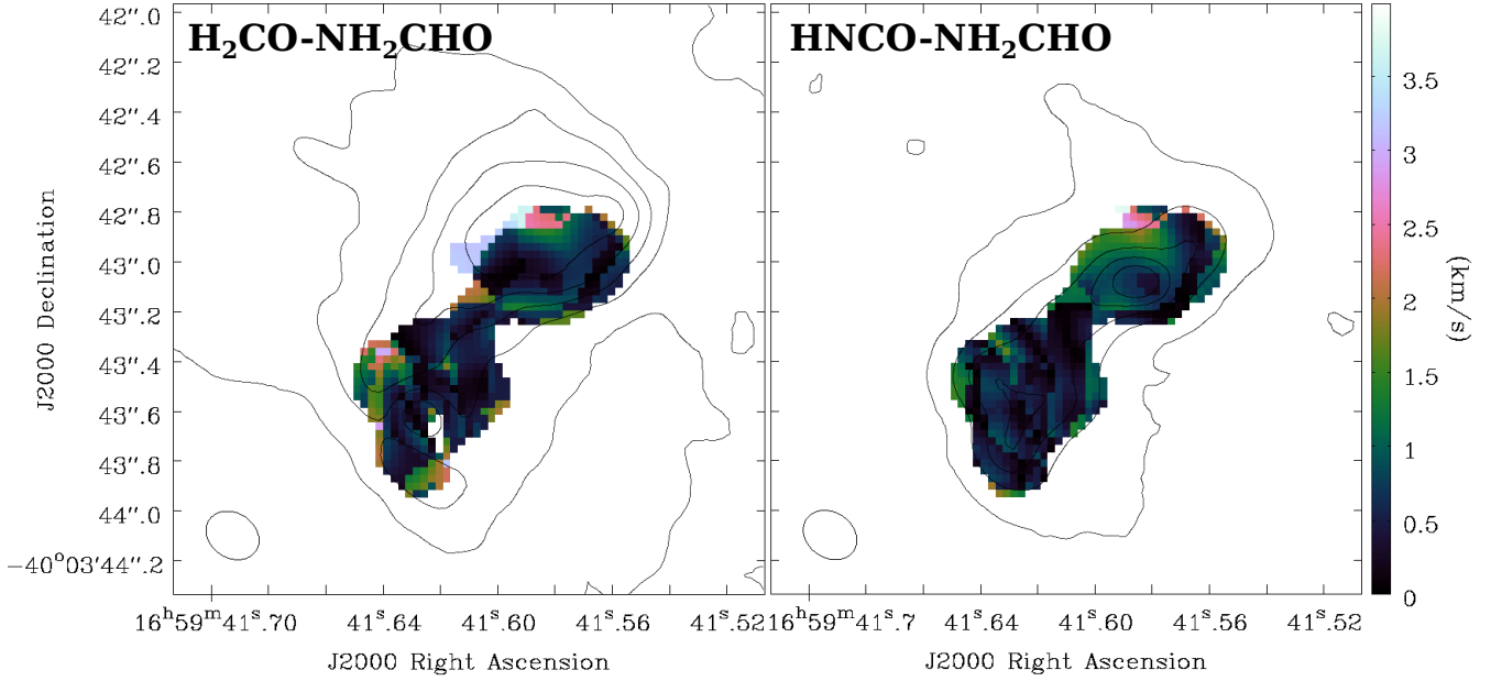
Fig. 11. Velocity difference (from first moment maps) at each pixel in G345 between ( left ) \text{H}_2\text{CO} (2) and \text{NH}_2\text{CHO} (1) and ( right ) \text{HNCO} (2) and \text{NH}_2\text{CHO} (1). The contours show the integrated intensity maps for \text{H}_2\text{CO} (2) and \text{HNCO} (2) as in Fig. 6. The velocity scale is the same for both panels.
