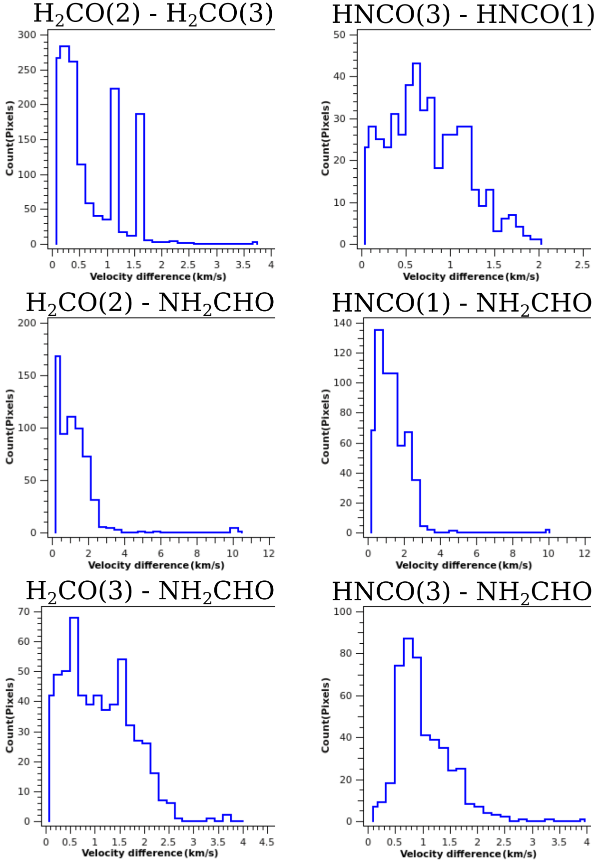
Fig. C.2. G24A1 first moment difference histogram.
