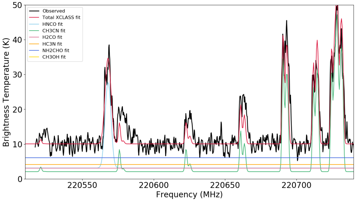
Fig. B.3. Spectral window from 220.5-220.75 GHz for G17 containing HNCO (2). We modeled two components for the CH 3 CN emission (green) toward this source.
