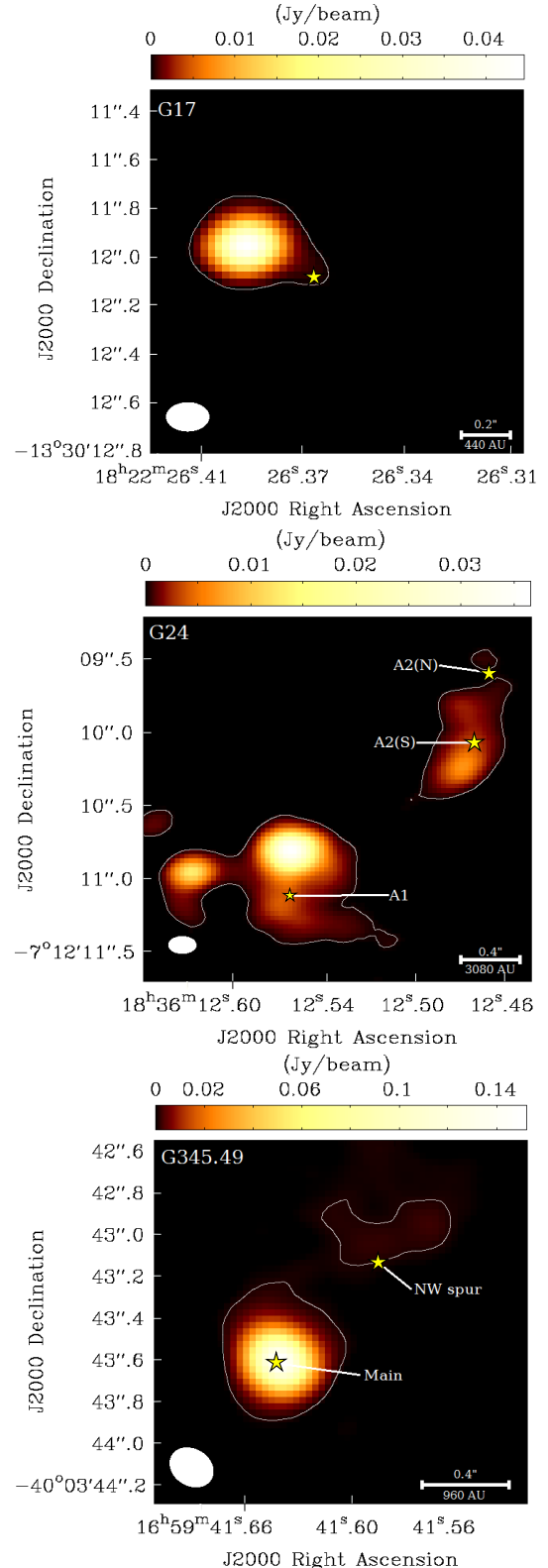
Fig. 1. Images of the 218 GHz continuum emission from Cycle 2 ALMA observations of our three regions focusing on the regions where \text{NH}_2\text{CHO} emission is observed. The color scale indicates the continuum flux as detailed in the color bar above each map. The white contour shows the 5\sigma contour levels for each panel: 1.5, 2.5, and 2.5 \text{mJy beam}^{-1} . The stars mark each of the spectral extraction points (coinciding with the zeroth moment peaks of \text{NH}_2\text{CHO} emission) and subsources are labeled.
