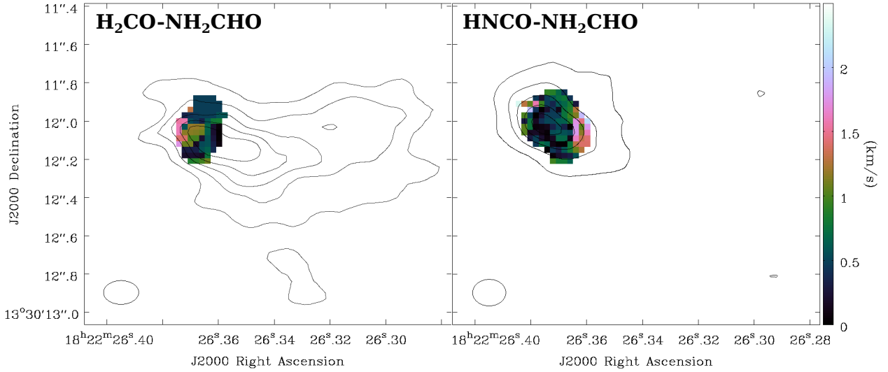
Fig. 9. Velocity difference (from first moment maps) at each pixel in G17 between ( left ) \text{H}_2\text{CO} (2) and \text{NH}_2\text{CHO} (1) and ( right ) \text{HNCO} (2) and \text{NH}_2\text{CHO} (1). The contours show the integrated intensity maps for \text{H}_2\text{CO} (2) and \text{HNCO} (2) as in Fig. 4. The velocity scale is the same for both panels.
