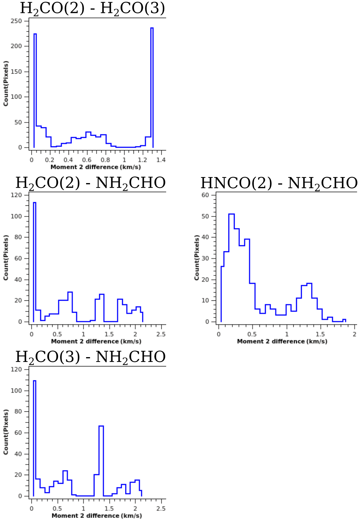
Fig. C.11. G345 Main second moment difference histogram.
