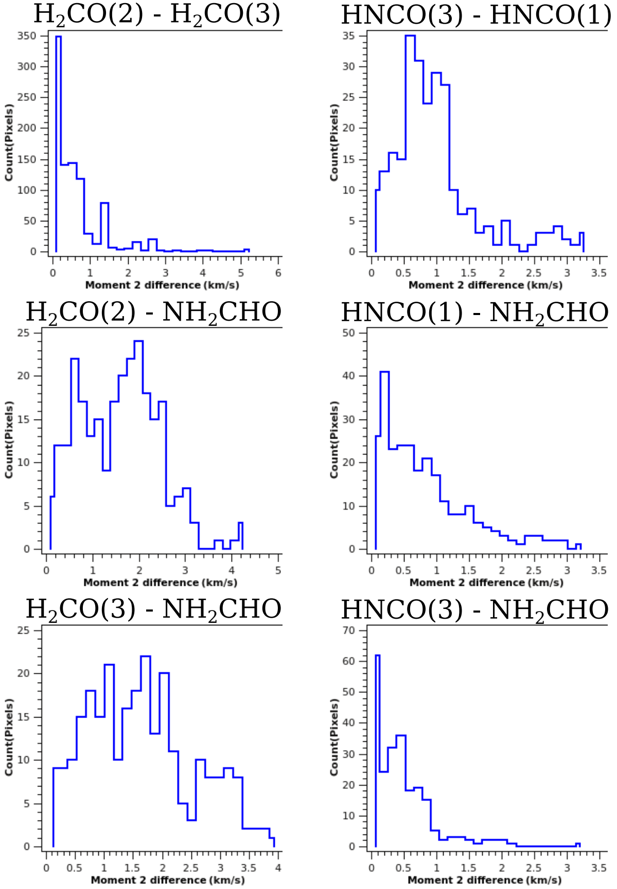
Fig. C.10. G24A2(S) second moment difference histogram.
