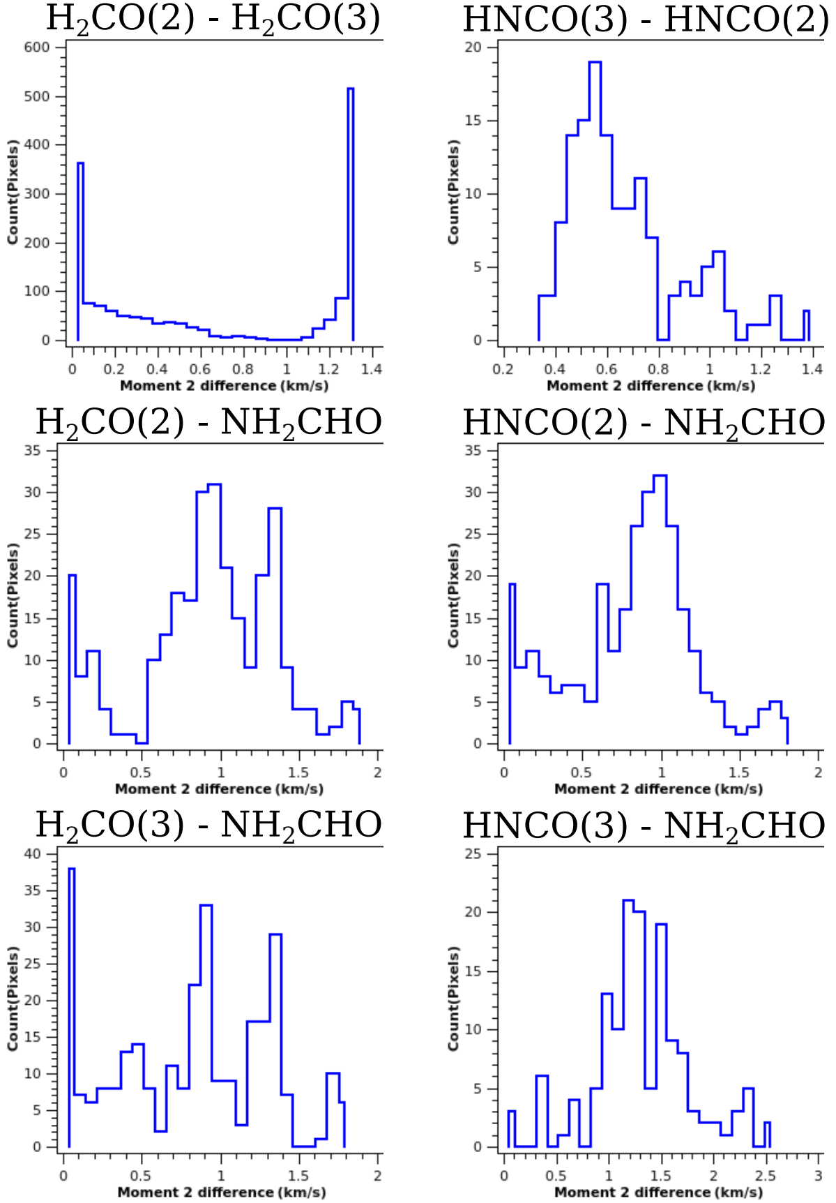
Fig. C.12. G345 NW spur second moment difference histogram.
