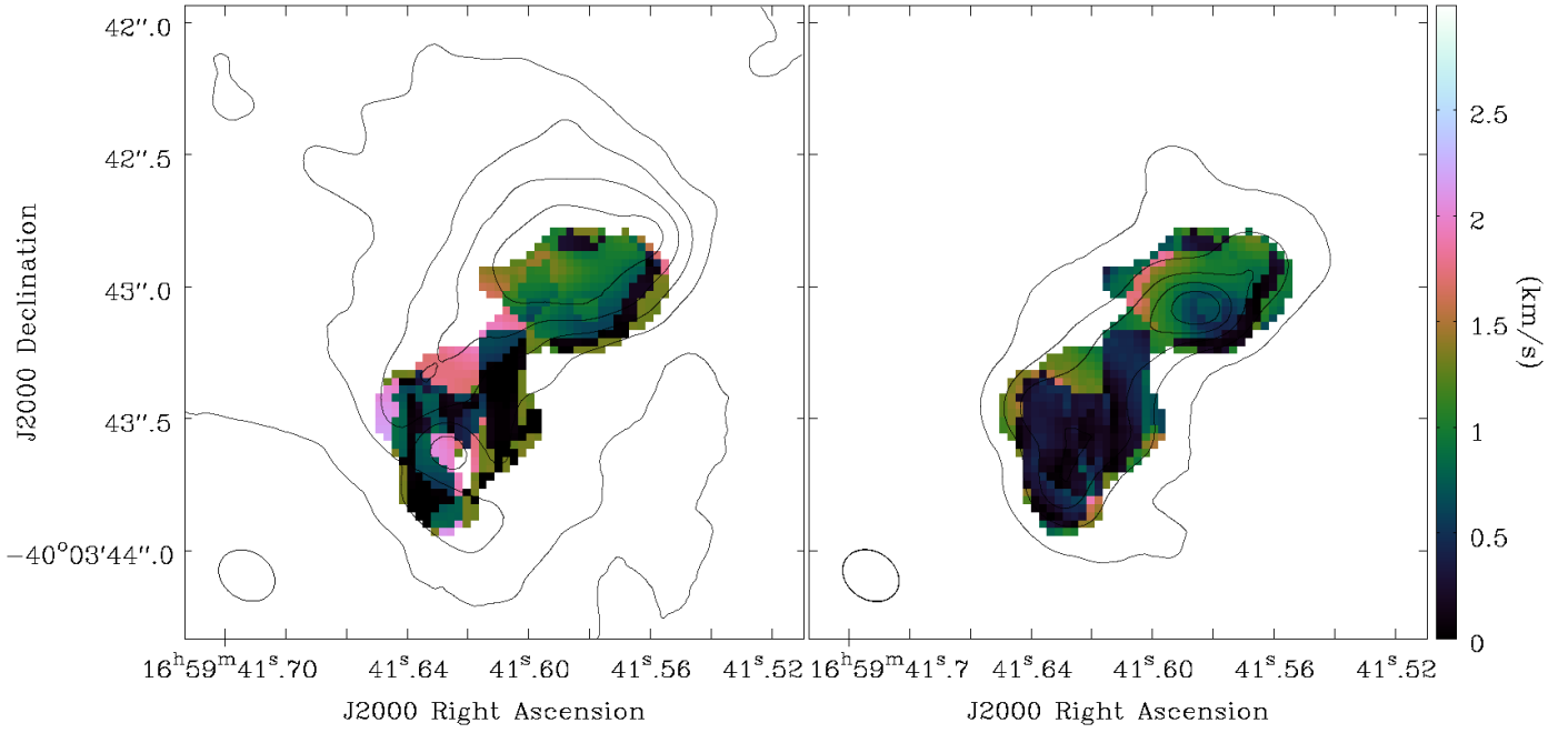
Fig. 15. Velocity dispersion difference (from second moment maps) at each pixel in G345 between ( left ) \text{H}_2\text{CO} (2) and \text{NH}_2\text{CHO} (1) and ( right ) \text{HNCO} (2) and \text{NH}_2\text{CHO} (1). The contours show the integrated intensity maps for \text{H}_2\text{CO} (2) and \text{HNCO} (2) as in Fig. 6. The velocity scale is the same for both panels.
