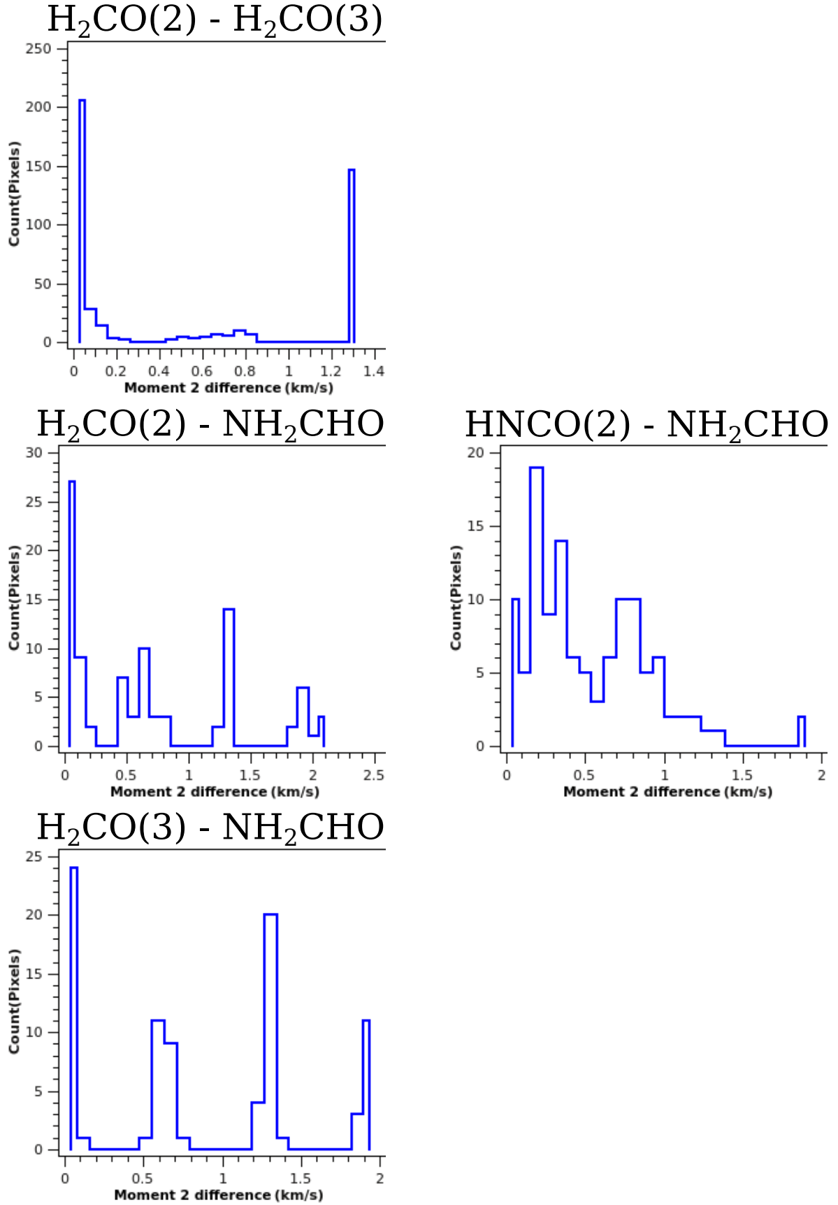
Fig. C.7. G17 second moment difference histogram.
