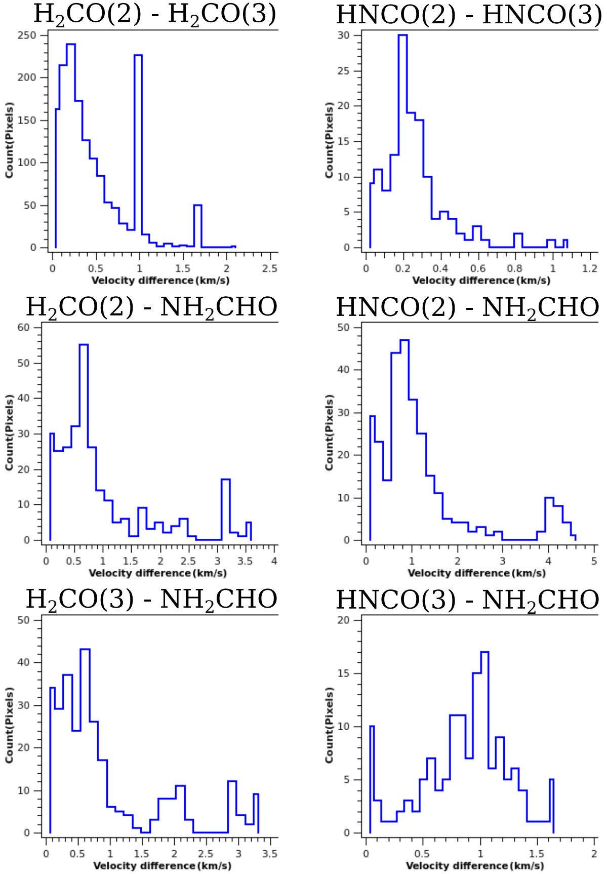
Fig. C.6. G345 NW spur first moment difference histogram.
