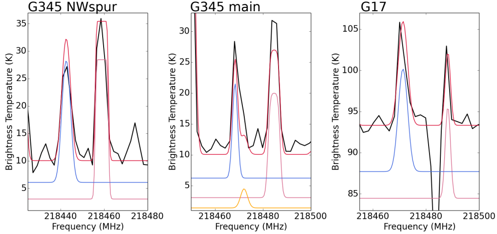
Fig. 3. Spectra with fits showing \text{NH}_2\text{CHO} (1) toward G345 NW spur (left), G345 Main (middle) and G17 (right). \text{NH}_2\text{CHO} (1) is weakly blended with \text{C}_2\text{H}_5\text{OH} in the spectra of G345 NW spur but unblended in G345 Main. The continuum levels are offset for easy viewing.
