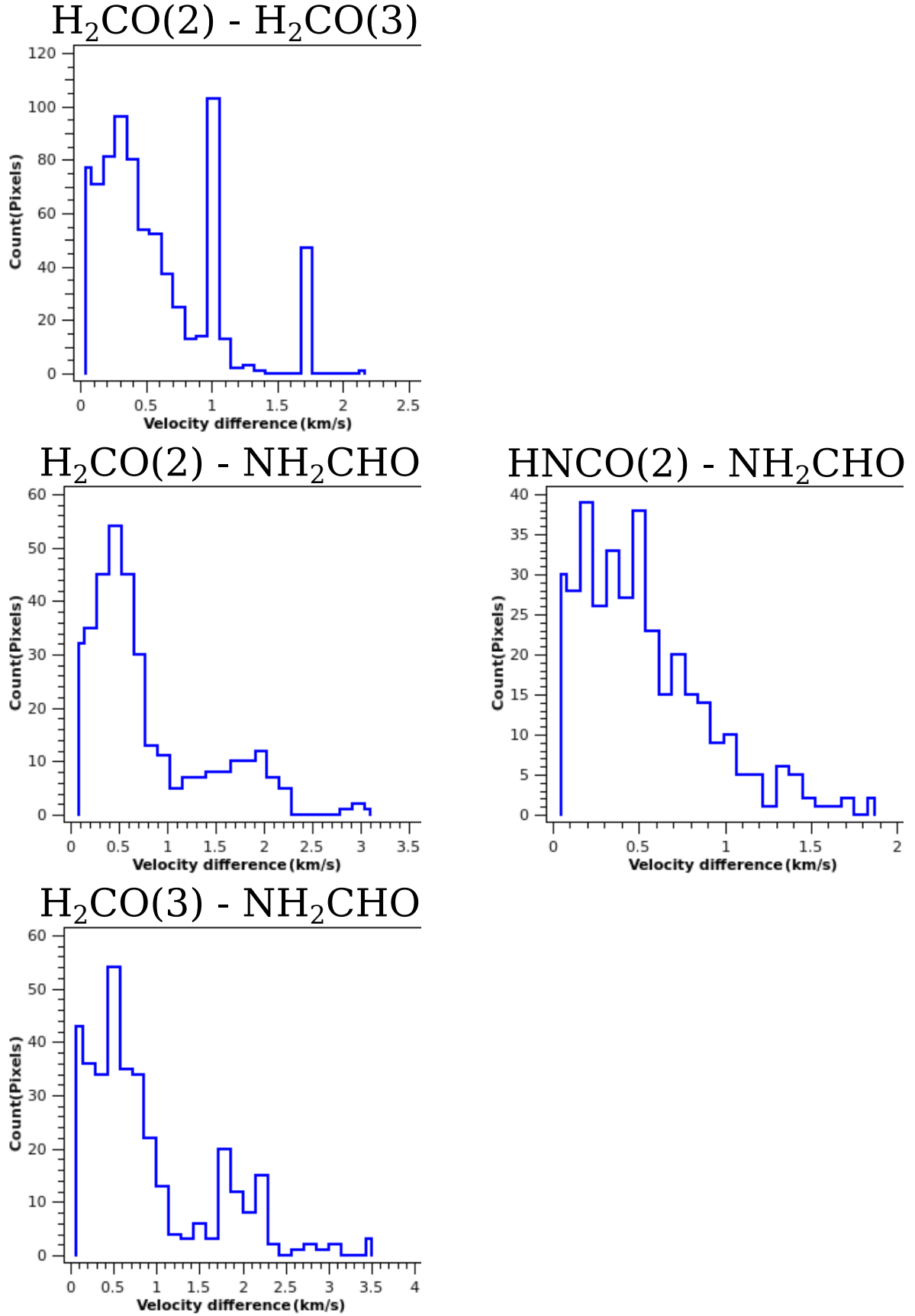
Fig. C.5. G345 Main first moment difference histogram.
