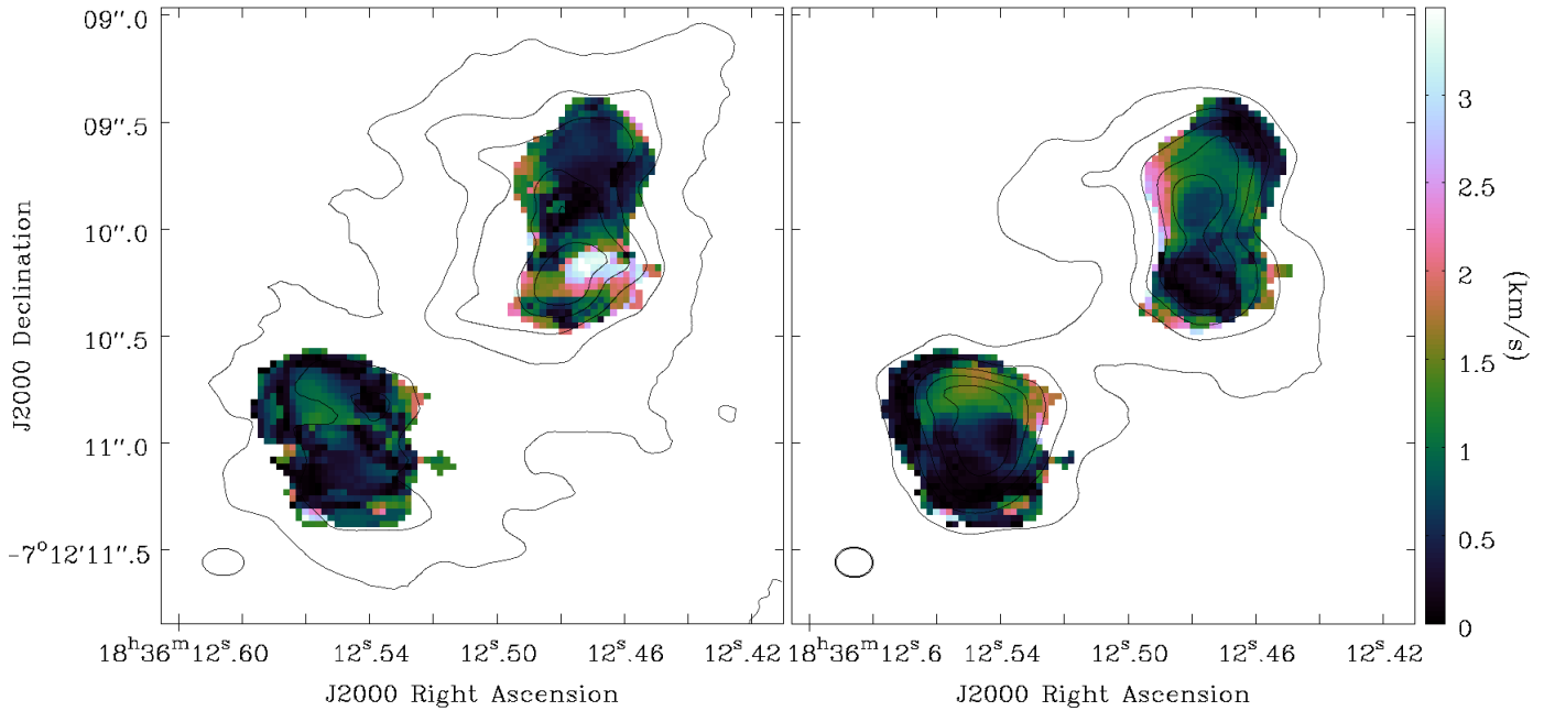
Fig. 14. Velocity dispersion difference (from second moment maps) at each pixel in G24 between ( left ) \text{H}_2\text{CO} (3) and \text{NH}_2\text{CHO} (2) and ( right ) \text{HNCO} (1) and \text{NH}_2\text{CHO} (2). The contours show the integrated intensity maps for \text{H}_2\text{CO} (3) and \text{HNCO} (1) as in Fig. 5. The velocity scale is the same for both panels.
