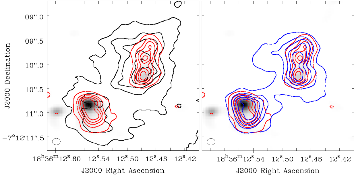
Fig. 5. G24 zeroth moment maps (contours) overlaid on the dust continuum (grayscale). Left: the black contours show the \text{H}_2\text{CO} (3) transition ( E_{\text{up}} = 68.1 K) from 5\sigma to a peak of 0.674 \text{ Jy beam}^{-1} \text{ km s}^{-1} (contour levels 0.03, 0.16, 0.29, 0.42, and 0.55 \text{ Jy beam}^{-1} \text{ km s}^{-1} ). The red contours show \text{NH}_2\text{CHO} (2) emission ( E_{\text{up}} = 78.9 K) from 5\sigma to 0.512 \text{ Jy beam}^{-1} \text{ km s}^{-1} (contour levels 0.026, 0.123, 0.220, 0.318, and 0.415 \text{ Jy beam}^{-1} \text{ km s}^{-1} ). Right: the blue contours show the extent of the \text{HNC} (1) emission ( E_{\text{up}} = 58.0 K) from 5\sigma to 0.738 \text{ Jy beam}^{-1} \text{ km s}^{-1} (contour levels 0.031, 0.172, 0.314, 0.455, and 0.597 \text{ Jy beam}^{-1} \text{ km s}^{-1} ) with the red contours showing \text{NH}_2\text{CHO} (as in the left frame).
