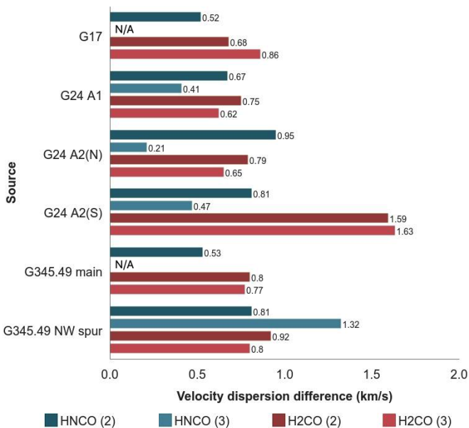
Fig. 12. Average velocity dispersion difference between \text{NH}_2\text{CHO} and transitions \text{HNCO} (2) and (3) and \text{H}_2\text{CO} (2) and (3). For the G24 sources \text{HNCO} (1) is used instead of \text{HNCO} (2).
