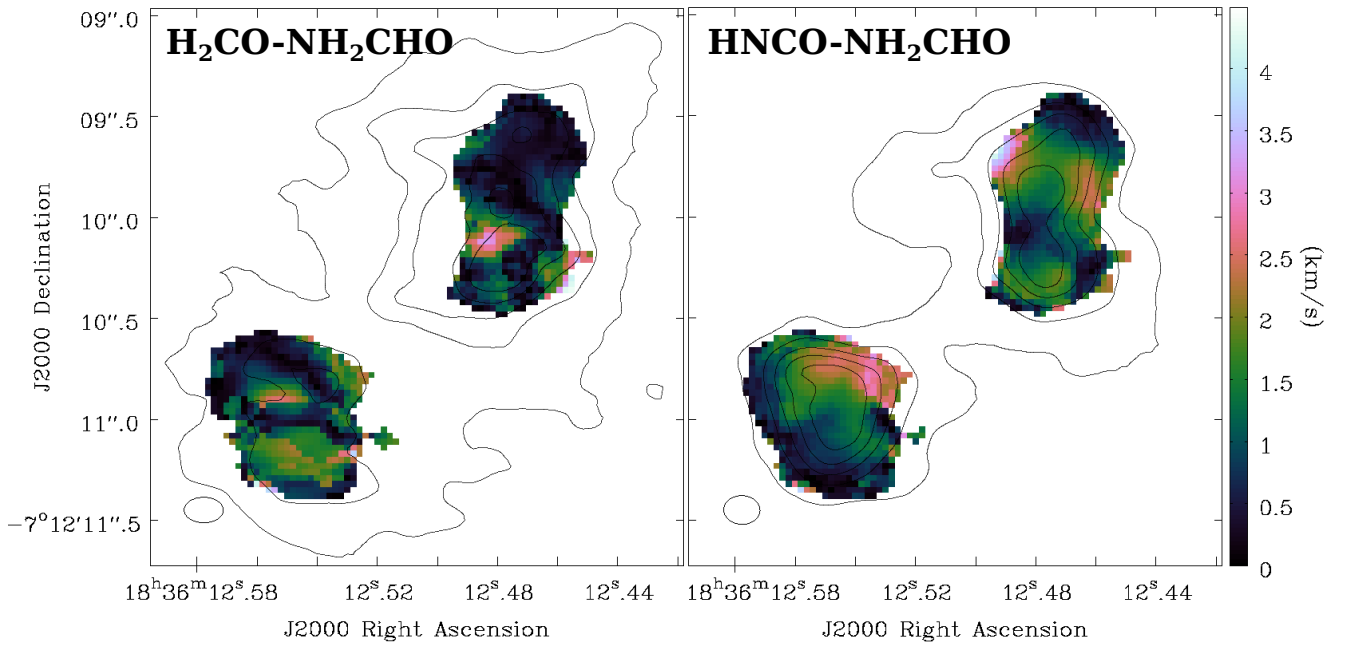
Fig. 10. Velocity difference (from first moment maps) at each pixel in G24 between ( left ) \text{H}_2\text{CO} (3) and \text{NH}_2\text{CHO} (2) and ( right ) \text{HNCO} (1) and \text{NH}_2\text{CHO} (2). The contours show the integrated intensity maps for \text{H}_2\text{CO} (3) and \text{HNCO} (1) as in Fig. 5. The velocity scale is the same for both panels.
