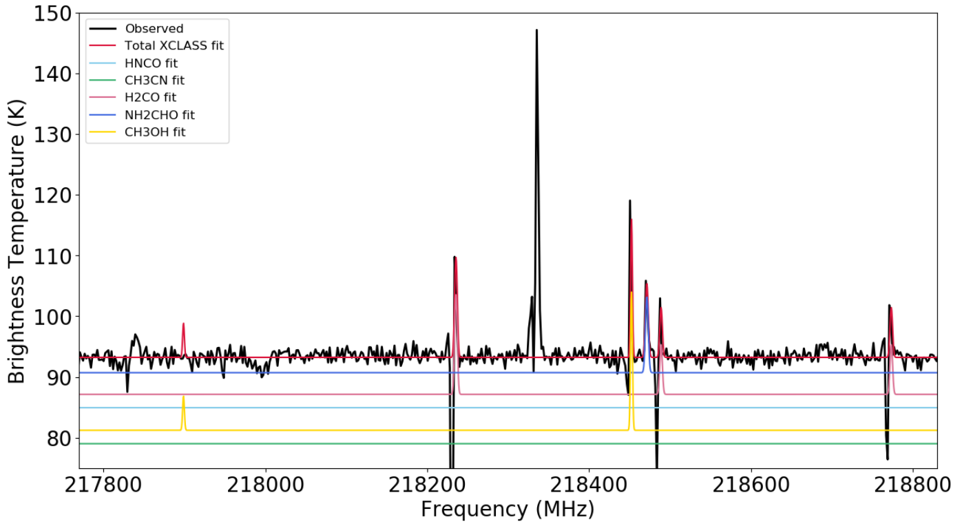
Fig. B.13. Spectral window from 217.8–218.8 GHz for G345 Main containing NH 2 CHO (1) and H 2 CO (1), (2), and (3).
