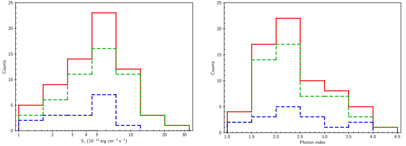
Fig. 4. Distribution of \gamma -ray energy flux ( left panel ) and photon index ( right panel ) above 10 GeV for the detected sources. Solid red line: all sources; green dashed line: Blazars; blue dashed line: UGS.
