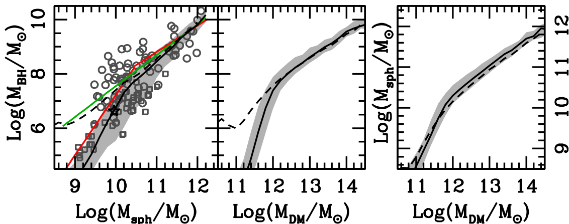
Figure 6. Additional black hole–spheroid scaling relations for z = 0 , for the different models considered in this work. Left-hand panel: M_{\text{bh}}-M_{\text{sph}} relation (data as in Fig. 2). Middle panel: M_{\text{BH}}-M_{\text{DM}} relation. Right-hand panel: M_{\text{sph}}-M_{\text{DM}} relation. In all panels, solid lines refer to the median relations in reference model (shaded areas representing the 5 and 95 per cent percentiles), while the dashed line to the corresponding \zeta_0 = 0 runs.
