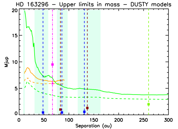
Figure 5. Same than Figure 4 but for mass limits obtained using DUSTY models.
