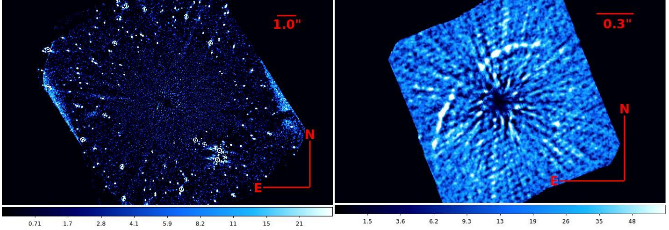
Figure 2. GLR maps obtained using PACO from the 2018-05-06 observations. In the left panel we display the IRDIS image while in the right panel we display the IFS image.
