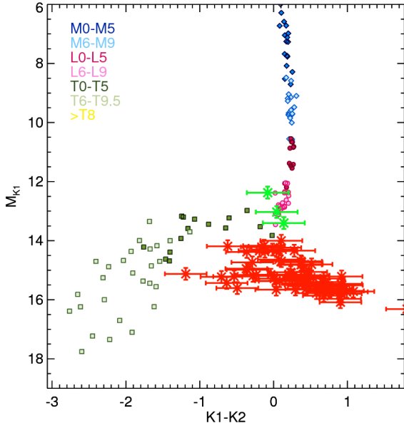
Figure 7. K1 versus K1-K2 color-magnitude diagram with the positions of the candidates detected in the HD 163296 IRDIS FOV for which it was not possible to apply the proper motion test. These objects are represented by red and green asterisks while squares and diamond with different colours represent field dwarfs with spectral types as indicated in the plot legend. Large part of these objects (red asterisks) are in a position of the diagram that confirm they are background objects. Three of them (green asterisks) are in a positions that does not allow a definitive conclusion about them.
