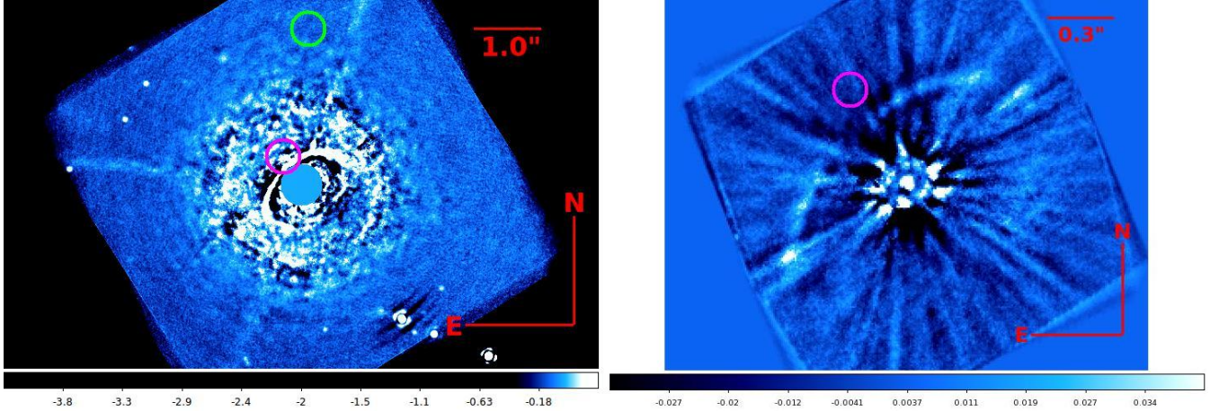
Figure 1. Final images obtained from the 2018-05-06 observations. In both cases the values are expressed in counts. Left: IRDIS final image obtained applying the PCA algorithm and subtracting 1 mode from the original data. The green circle is to enlight the zone around the planet proposed by Pinte et al. (2018) , the magenta circle enlight the zone of the planet proposed by Guidi et al. (2018) . The mask covering the star has a radius of 0.37'' . Right: IFS final image obtained using the PCA algorithm subtracting 1 mode from the original data. As for the IRDIS image, the magenta circle identify the zone around the planet proposed by Guidi et al. (2018) .
