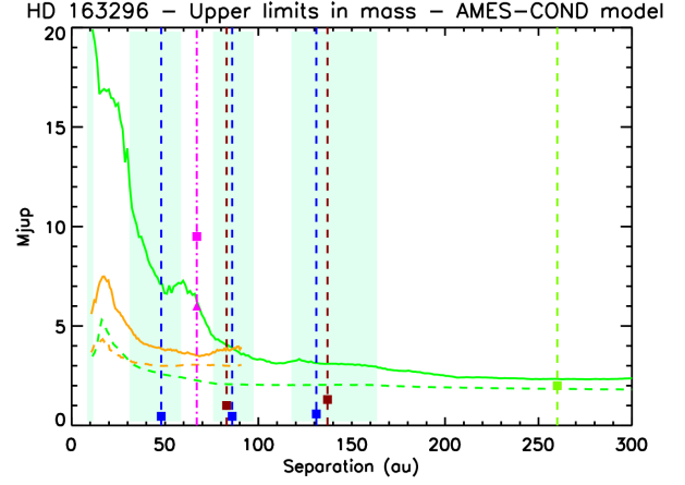
Figure 4. Mass limits versus the separation from the central star expressed in au for IRDIS (green line) and for IFS (orange line) obtained using the AMES-COND models. The dashed lines in the same colours represents the mass limits obtained using PACO. The light cyan areas represent the estimated positions of the gaps around the star as estimated in Isella et al. (2018) . We also overplot the dashed lines that represent the positions of the planets proposed by Liu et al. (2018) (blue lines), Teague et al. (2018) (red lines), Pinte et al. (2018) (green line) and Guidi et al. (2018) (magenta line). Further, we added the foreseen mass of each proposed planet denoting them with a filled square of the same color of the corresponding line. In the case of the planet proposed by Guidi et al. (2018) we used a filled triangle to show the mass of the planet as proposed in the paper and the updated value of planetary mass with a filled square (see the text for more details).
