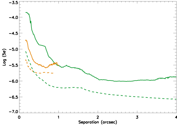
Figure 3. 5\sigma contrast vs separation expressed in arcsec obtained for IRDIS (solid green line) and for IFS (solid orange line) using the PCA algorithm and subtracting 1 mode from the original data as done for the images shown in Figure 1. The dashed lines represent the contrast obtained using PACO using patch radii of 4 and 5 pixels for K1 and K2 filters respectively.
