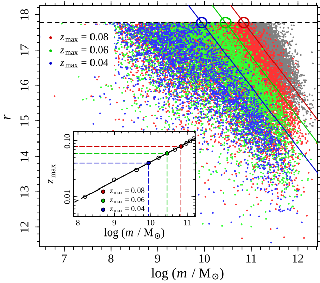
Figure 2. Illustration of the estimation of maximum redshift for completeness at a given stellar mass (for the STARLIGHT / V15 model, see Table 1). Main plot: apparent magnitude versus stellar mass, for SDSS galaxies in the clean sample, whose r = 17.77 flux limit is shown as the dashed horizontal line. The full set of galaxies is shown in grey, with galaxies at three representative redshifts, z = 0.04, 0.06 , and 0.08 , shown in blue, green, and red, respectively, for illustrative purposes, with the corresponding oblique coloured lines representing our estimates of 95th percentiles of mass as a function of apparent magnitude, for that maximum redshift. The large coloured circles indicate the values of m_{95}(r_{\text{lim}}) . Inset: resultant maximum redshift versus stellar mass (with same colour code), with the three representative redshifts and corresponding masses shown in colour.
