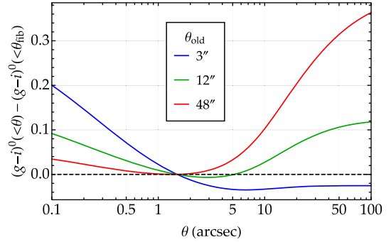
Figure 22. Colour profiles for a mixed population of young and old stars, with n_{\text{old}} = 3 and other parameters from Table 3.
