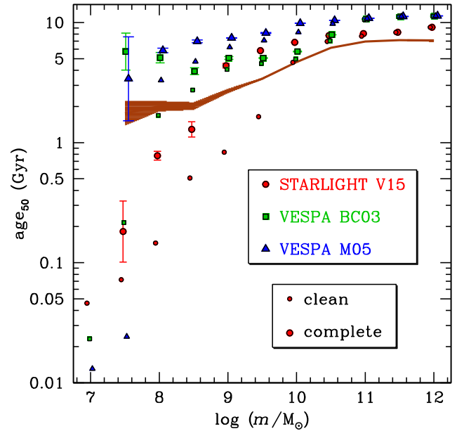
Figure 8. Median (over galaxies within a given mass bin) of ‘median’ stellar ages versus stellar mass for galaxies in the clean (small symbols) and complete (large symbols) SDSS Main Galaxy Sample according to STARLIGHT with the Vaz15 model (red circles), VESPA with BC03 (green squares) and VESPA with Maraston et al. (2005, blue triangles). The brown shaded region shows the mass-weighted arithmetic mean ages from the intersection of the Gallazzi et al. (2005) sample with the complete sample. The error bars (only shown for the complete sample) and the widths of the shaded regions are the uncertainties on the medians from 100 bootstraps.
