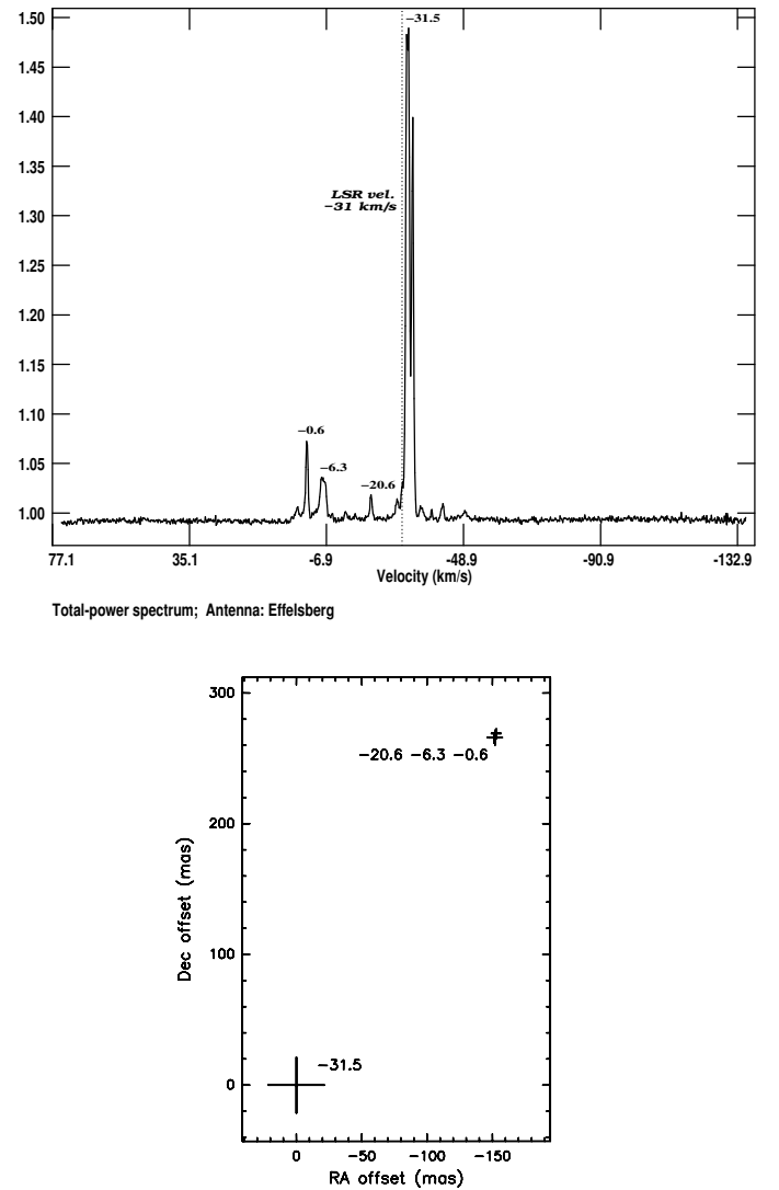
Fig. 4. Upper: Effelsberg total power spectrum for NGC281-W. The vertical dotted line indicates the systemic LSR velocity. The labels indicate the velocities in [\text{km/s}] of the most prominent features, for which we have made maps. Lower: Distribution of \text{H}_2\text{O} maser spots corresponding to the dominant emission features in the total power spectrum. The channel with the highest emission (vel. -31.5 \text{ km s}^{-1} ) was used as reference in the astrometric analysis. The labels in the plot indicate the velocities corresponding to each spot, in [\text{km/s}] ; the size of the crosses is proportional to the square root of the peak flux in the maps.
