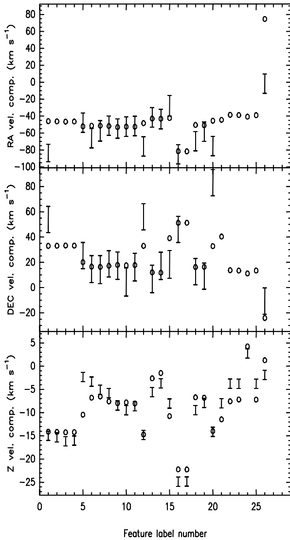
Fig. 3. Comparison between the observed maser velocity components and those obtained from the best model fit, for data from global multi-epoch VLBI observations.
