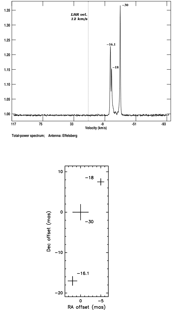
Fig. 5. Upper: Effelsberg total power spectrum for GGD12-15. The vertical dotted line indicates the systemic LSR velocity. The labels indicate the velocities in [km/s] of the most prominent features, for which we have made maps. Lower: Distribution of H 2 O maser spots corresponding to the dominant emission features in the total power spectrum. The channel with the highest emission (vel. -30 \text{ km s}^{-1} ) was used as reference in the astrometric analysis. The labels in the plot indicate the velocities corresponding to each spot, in [km/s]; the size of the crosses is proportional to the square root of the peak flux in the maps.
