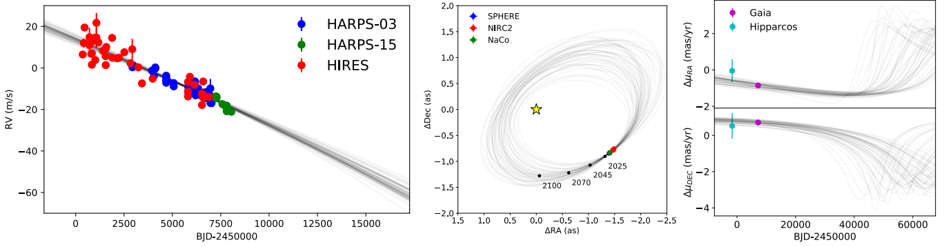
Fig. 8. Sample of 50 model orbits (gray curves) fitted on the HD 19467B data (colored points) from RV (left), imaging (middle), and astrometry (right). In the middle panel, the yellow star marks the location of the star and the black dots show the median predicted position for a few epochs in the future.
