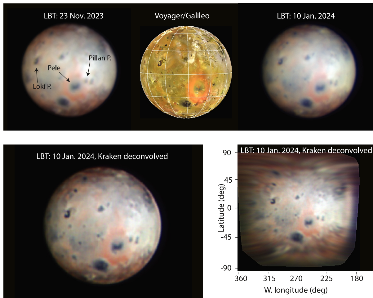
Figure 2. The SHARK-VIS detection image on 23 November 2023 (upper left), on 10 January 2024 (upper right), and the reprojection of the Voyager and Galileo spacecraft-derived Io photomosaic for 10 January 2024 (center) (Becker & Geissler, 2005). Labels to Pele, Pillan Patera and Loki Patera are shown on the upper left image. The bottom row shows the Kraken-deconvolved image from 10 January 2024 on the left; the bottom right map shows this image reprojected onto equirectangular (approximate) longitude-latitude coordinates. All images have been rotated so Io North is up. No detectable change to the Pillan plume deposit has occurred during the 50 days separating the two observations.
