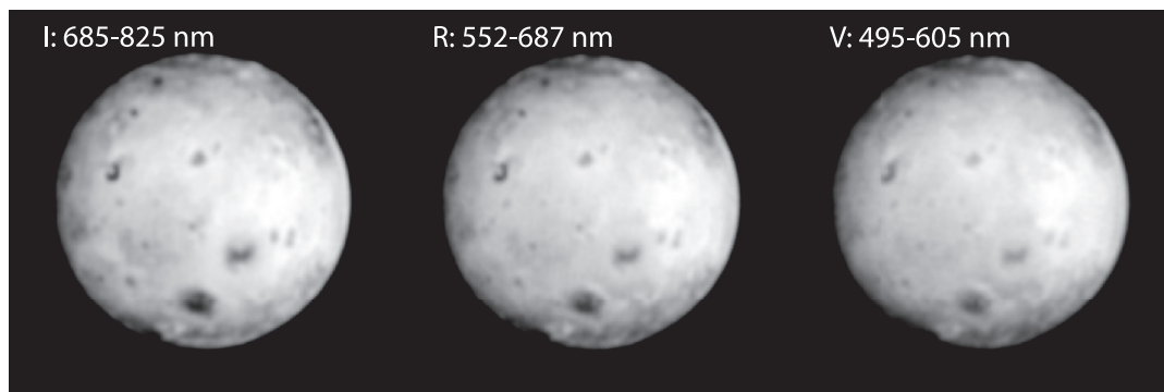
Figure 1. Images of Io obtained with SHARK-VIS on the LBT in November 2023 and January 2024. The images are re-scaled to Io's apparent diameter. The third row shows the Kraken deconvolved images from January 2024. The filter used is shown on each image. Io North is approximately up.
