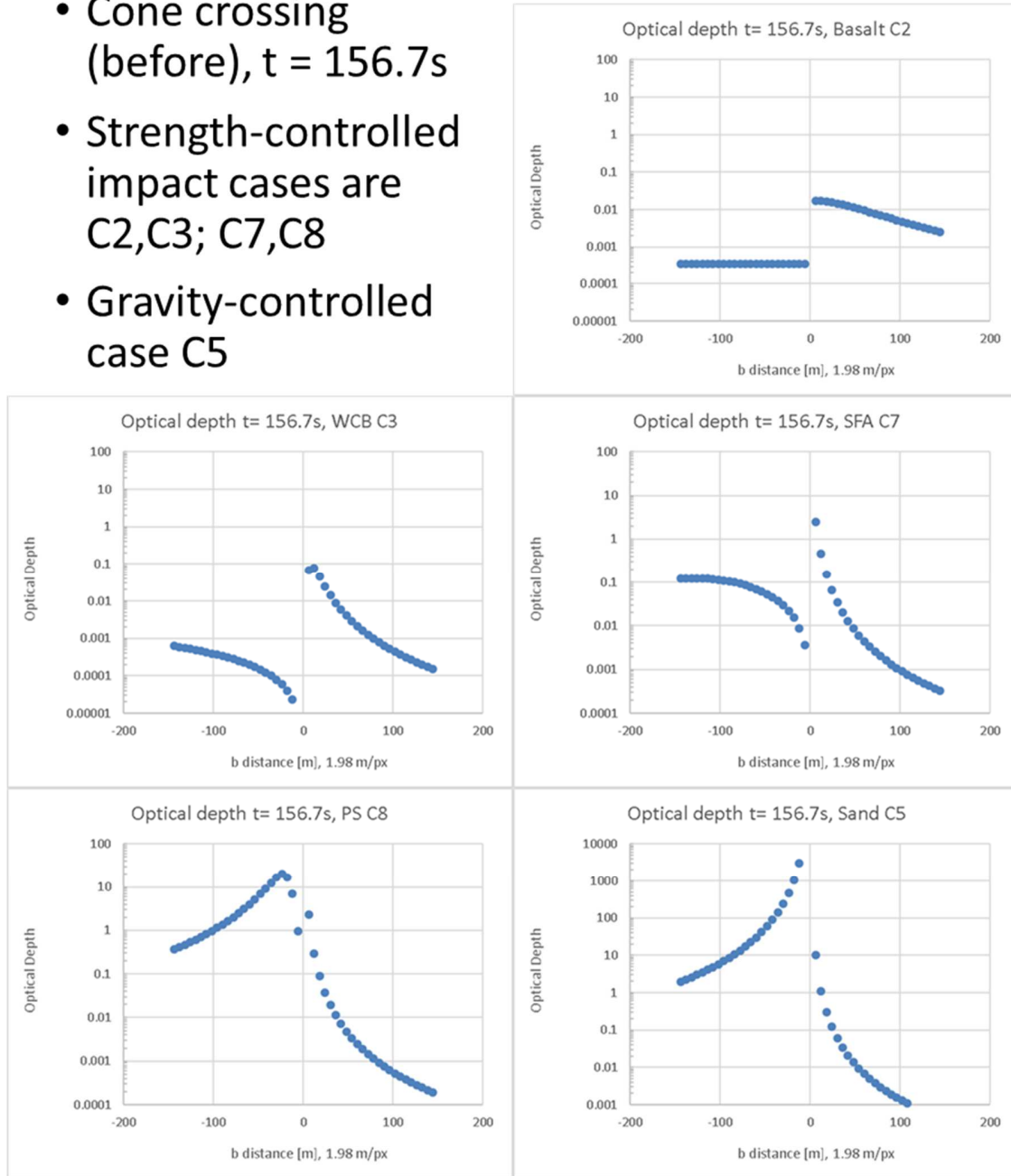
Figure 13. Same as Fig. 7 but at time t=156.7\text{ s} , where \alpha + \varepsilon = 46.171^\circ . Close to time of ejecta cone crossing; maximal effect of obliquity enables estimation of ejecta cone thickness. Obliquity effect for case C5 reduces \tau over one limb of target body, even though clearing has not yet begun.
