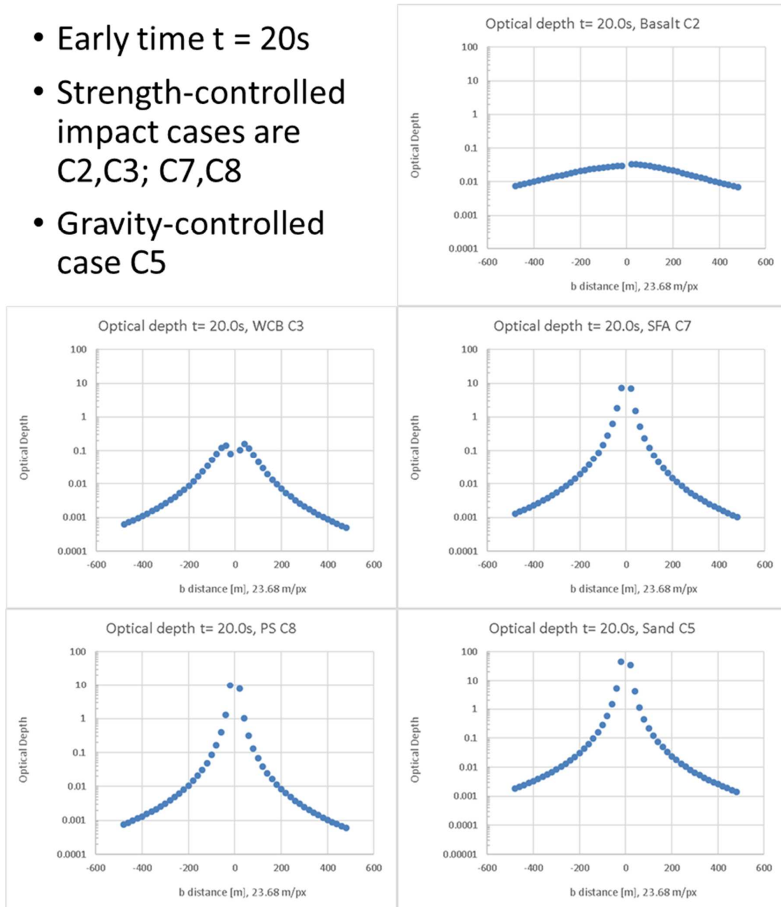
Figure 9. Same as Fig. 7, at time t=20\text{ s} after DART impact, where \alpha + \varepsilon = 86.686^\circ . Compared to Figs. 7 and 8, clearing of plume optical depth continues for C2 and begins for C3. In weak target cases (bottom row), optical depth is increasing with time at all distances plotted.
