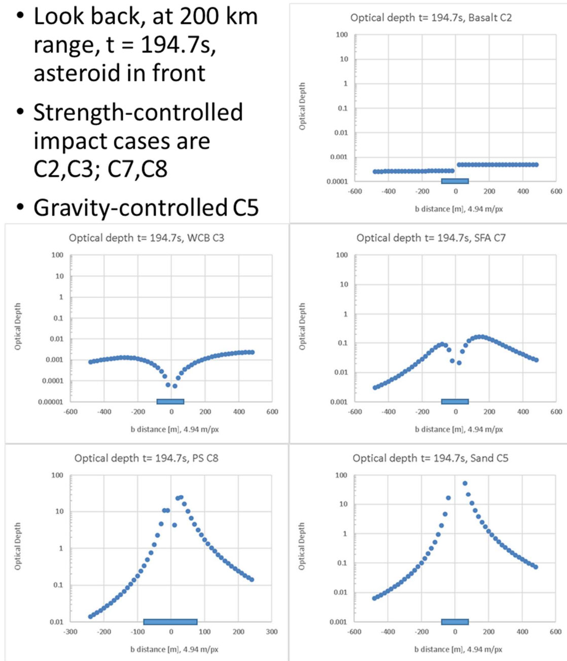
Figure 15. Same as Fig. 7 but at time t=194.7\text{ s} , after closest approach, where \alpha + \varepsilon = -73.918^\circ . Plume is imaged above the limb of the target body, in forward scattering geometry at 120^\circ phase angle. Region behind asteroid indicated by 160 m scale bars.
