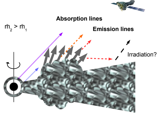
Figure 12. Simplified scheme of a variable high mass accretion rate source. The compact object is surrounded by an inner corona (or accretion column) and a thick disc of matter from the companion star. Left panel: Above the Eddington limit ( \dot{m}_1 > \dot{m}_E ) radiation pressure thickens the disc and launches a powerful wind from a region around the spherisation radius ( R \sim 25 R_S for v_{\text{esc}} \sim 0.2c ). Right panel: At even higher accretion rates ( \dot{m}_2 > \dot{m}_1 > \dot{m}_E ), the source simultaneously brightens and softens, the spherisation radius extends to larger radii and a cooler phase of the wind is launched at larger radii ( \sim 150 R_S for 0.08c ). The emission lines, presumably coming from the outer irradiated disc, also become stronger and broader. These trends are observed in NGC 1313 X-1.
