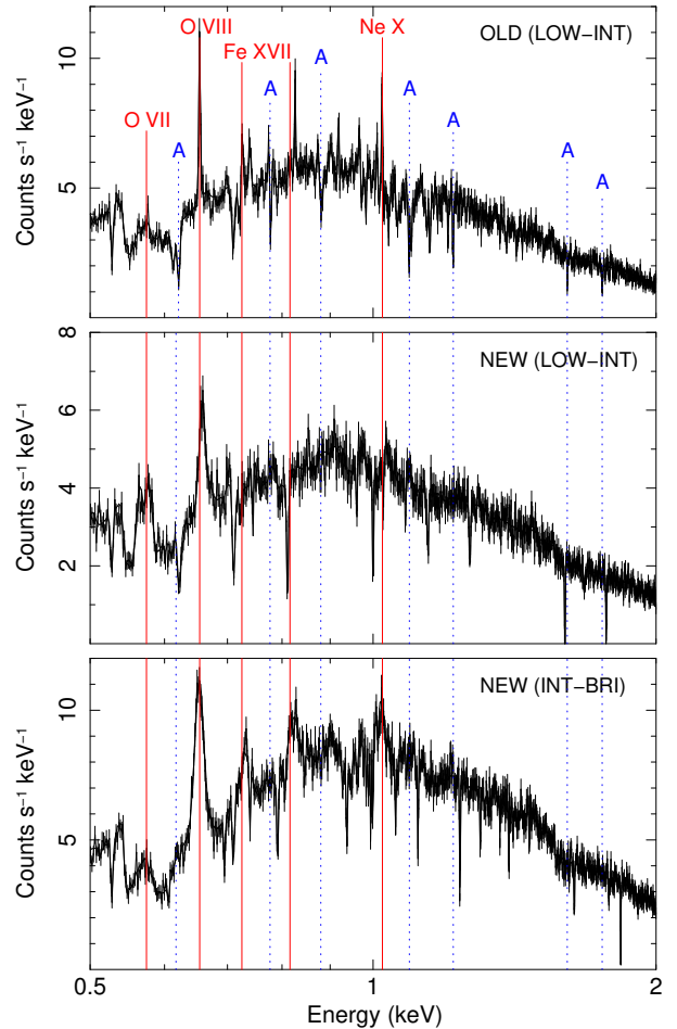
Figure 13. ATHENA / X-IFU simulations of the ULX NGC 1313 X-1 for the three spectra with overlaid the best-fit multiphase wind model. The wind model consists of photoionised emitting plasma and a two-phase absorber (see Table A1 and Fig. A2). Cosmic X-ray background and particle background are accounted for. The X-IFU response matrix is dated 10/2018 with 1.4 \text{ m}^2 effective area at 1 keV. Note how the lines strongly differ in these spectra.
