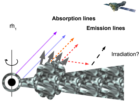
Figure 12. Simplified scheme of a variable high mass accretion rate source. The compact object is surrounded by an inner corona (or accretion column) and a thick disc of matter from the companion star. Left panel: Above the Eddington limit ( \dot{m}_1 > \dot{m}_E ) radiation pressure thickens the disc and launches a powerful wind from a region around the spherisation radius ( R \sim 25 R_S for v_{\text{esc}} \sim 0.2c ). Right panel: At even higher accretion rates ( \dot{m}_2 > \dot{m}_1 > \dot{m}_E ), the source simultaneously brightens and softens, the spherisation radius extends to larger radii and a cooler phase of the wind is launched at larger radii ( \sim 150 R_S for 0.08c ). The emission lines, presumably coming from the outer irradiated disc, also become stronger and broader. These trends are observed in NGC 1313 X-1.
