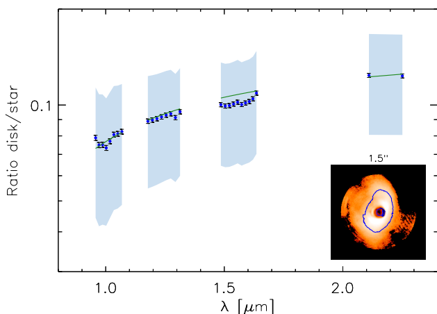
Fig. 6. Disk mean spectrum of HD 100546 along the wings. The blue dots and the shaded regions refers to the median value and its 3\sigma uncertainty. The green line represent the best fit obtained with light reflected by dust with constant albedo A = 0.65 . In the bottom-right inset, the area selected for the spectrum extraction on the RDI images is delimited in blue.
