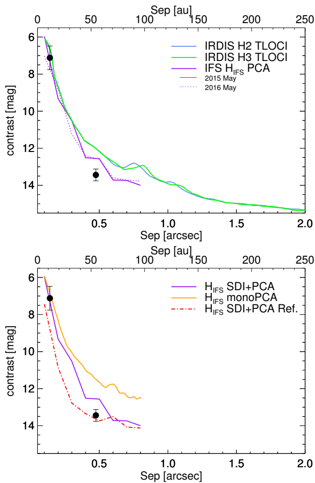
Fig. 10. Top: contrast curves for HD 100546 obtained in the H_{IFS} band for the two best IFS datasets applying SDI+PCA and for IRDIS H2H3 dataset applying TLOCI. Bottom: The IFS May 2015 contrast curve shown above is compared with the result obtained with 2 modes monochromatic PCA (orange curve) and with the contrast curve in the H_{IFS} band for HD 95086 applying SDI+PCA (in red dashed-dotted line). The planets contrast values measured in the H band obtained by Currie et al. 2015 with GPI are reported in both panels.
