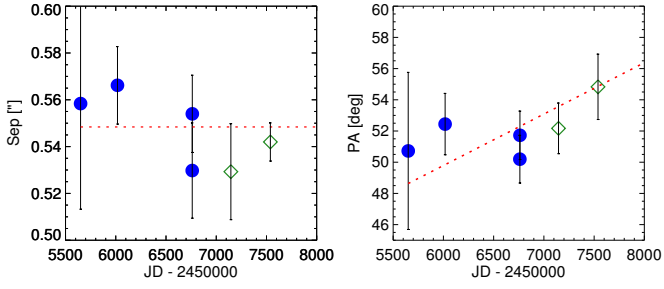
Fig. 12. Run of deprojected separation (left panel) and of position angle (right panel) of CCB with time. Data are from Quanz et al. (2013); Currie et al. (2014); Quanz et al. (2015) (blue dots) and this paper (open diamonds). Dashed lines are predictions for a circular orbit on the plane of the disk.
