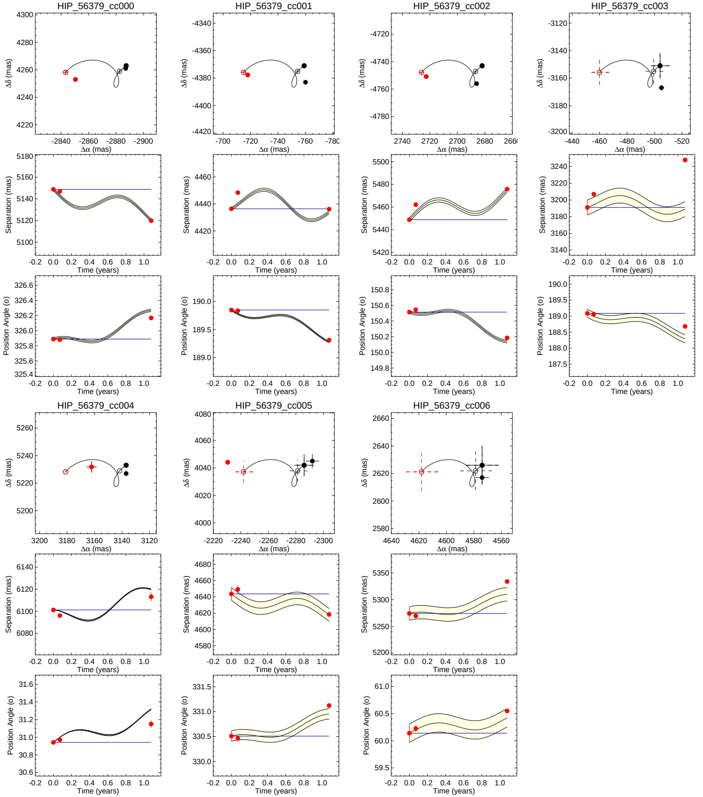
Fig. A.1. Top panel: proper motion in \alpha and \delta of the background objects in the IRDIS FoV of HD100546 considering data from 4 May 2015 (filled black), May 29th 2015 (open black), May 31st 2016 (filled red). Dotted points and errorbars represent the expected position for a background object. Middle panel: observed time variation of the separation compared with the expected one for a background object. Bottom panel: observed time variation of the position angle compared with the expected one for a background object.
