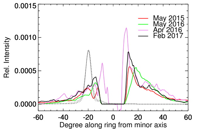
Fig. 11. Intensity profile as a function of phase of the two wings at different epochs. Phase 0 correspond to the near side of the semi-minor axis and negative values correspond to the SE wing. The dashed profile correspond to a point like source located at the expected position of CCc crossing the ring with the contrast upper limit given by Currie et al. (2015). April 2016 data set was scaled by an arbitrary factor of 1.6 to overlap other profiles.
