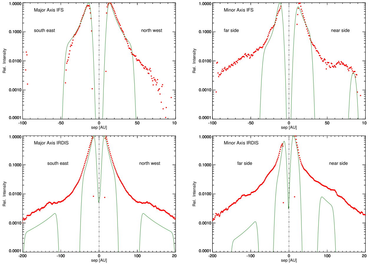
Fig. 7. Radial profile along the semi-major and the semi-minor axis of HD 100546 RDI images (red dots) compared with the best fit model (green line) obtained for IFS and IRDIS.
