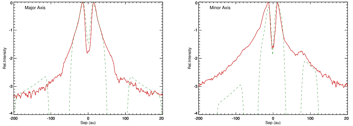
Fig. 8. Radial profile along the semi-major and the semi-minor axis of HD 100546 PDI images (continuum line) compared with the best fit model (dashed line) IRDIS.
