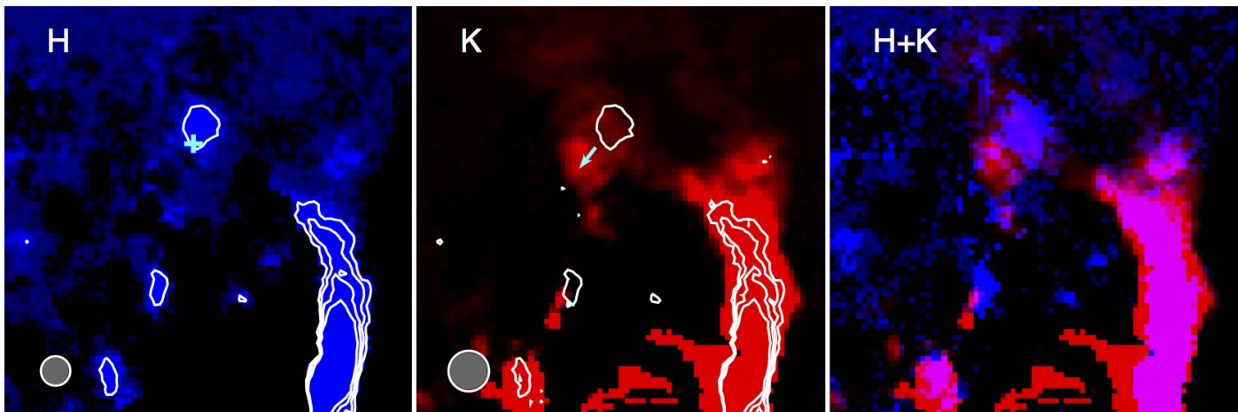
Fig. 13. Comparison of HD 100546 images in different band filters. One component PCA images of IRDIS H2H3 taken on May 29th 2015 (left), K1K2 taken on May 3rd 2015 (middle) and their combination (right). Contours refer to IRDIS H2H3. The cross represents Currie et al. (2015) detection in GPI H band, the arrow in the central panel indicate the motion of CCB between Quanz et al. (2015) detection in NACO L' band and our May 2016 K1K2 detection of CCB. The grey circle represent the resolution element of the images.
