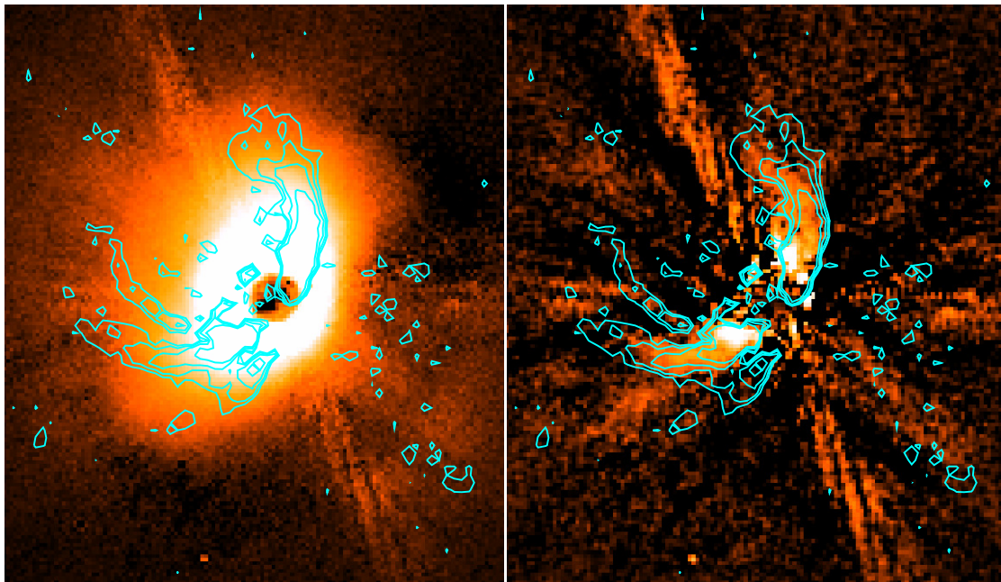
Fig. 5. IRDIS PDI J band Q_\phi image (left) and the results of a simulated cADI analysis on this image. Overplotted in cyan the isophotes of IRDIS cADI H2 observations.
