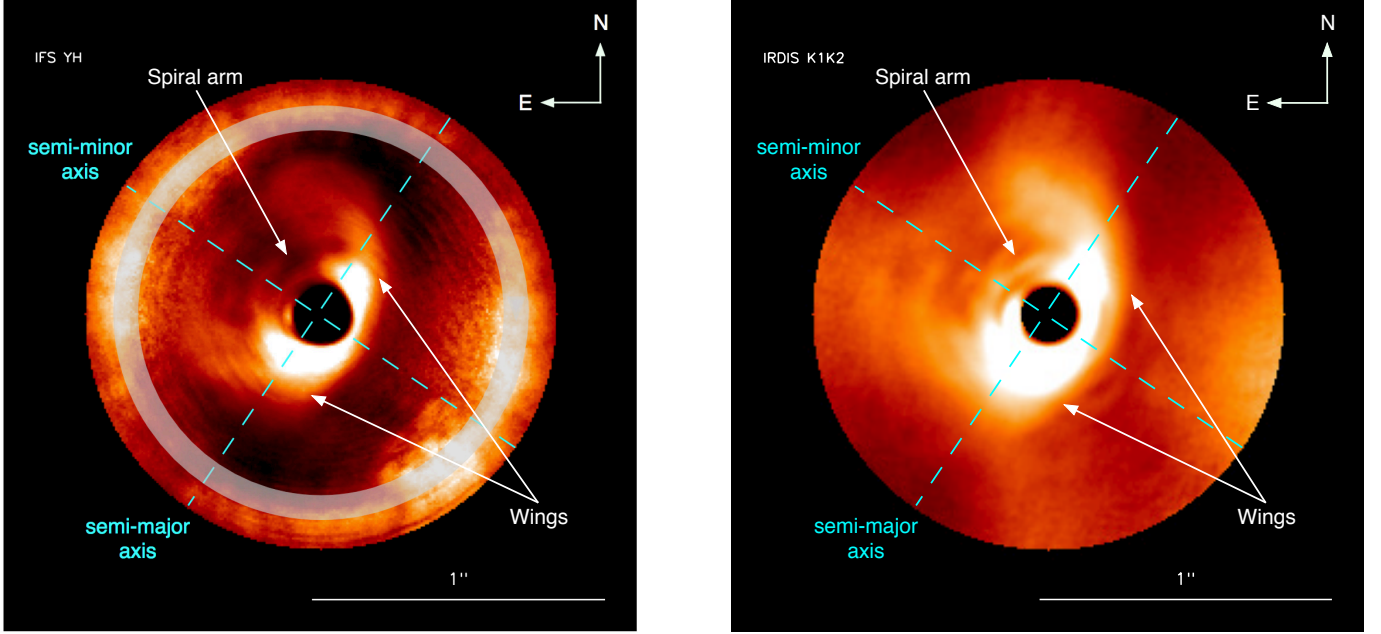
Fig. 2. May 2015 IFS collapsed YH (left) and IRDIS K1K2 (right) results for HD100546 using RDI. Both images are r^2 -scaled to also enhance structures at larger radii. The grey circle in the left image indicate the SPHERE AO control radius at r \approx 20 \times \lambda/D .
