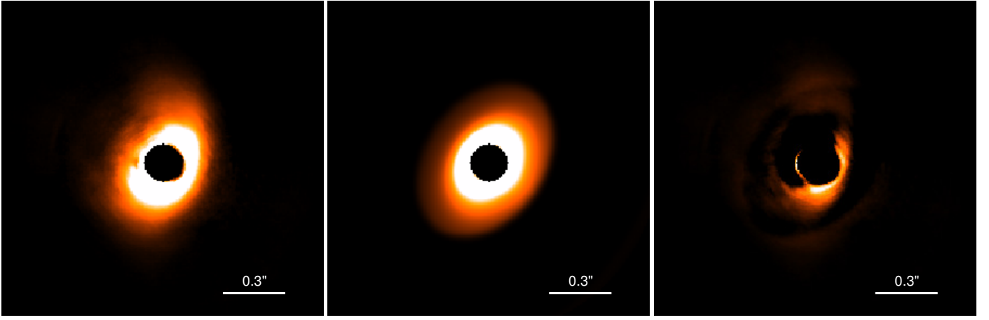
Fig. 9. From left to right, IFS RDI image, model and residuals. Image are displayed with the same linear color bar from 6 \times 10^{-3} dex to 1 dex. North is up, East is left.
