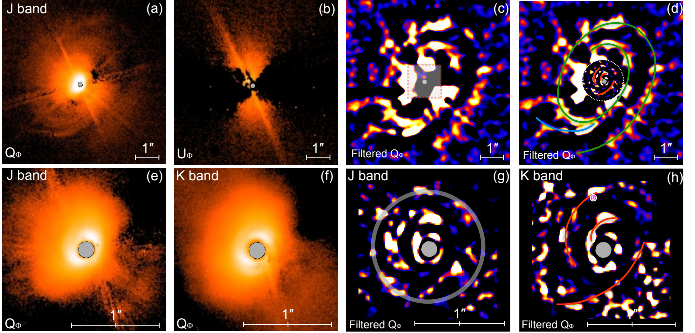
Fig. 4. Polarized light images of HD100546 from SPHERE/IRDIS. (a): The Q_\phi image in the J band. (b): The U_\phi image in the J band. (c): Unsharp masking of the Q_\phi image in the J band (see text). The inner box defines the region displayed in the bottom row. (d): Labeled version of (c). The inner inset circle is from (g). (e): Inner detail of the Q_\phi image in the J band. (f): Inner detail of the Q_\phi image in the K band. (g): Unsharp masking (see text) of (e). The grey circle indicates the IRDIS control radius at r \approx 20 \times \lambda/D (see text). (h): Unsharp masking (see text) of (f). Features visible from both (g) and (h) are labeled. The purple dot indicates the location of CCb from Quanz et al. (2013). In all images, the central star is in the middle of the grey circle, symbolizing the instrument coronagraphic mask. The logarithmic color stretch is relatively arbitrary and refers to positive values, except in (a) and (b) where it is the same. North is up, East is left.
