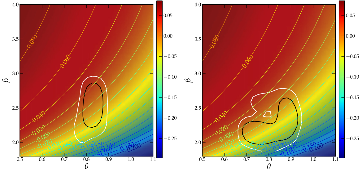
Figure 19. Magnitude difference (measured in 3'' diameter apertures) between a point-like object convolved with the target PSF \mathcal{M}[0''.8, 2.5] and with \mathcal{M}[\theta, \beta] in the 2D parameter space [\theta'', \beta] . The black and white contours represent the regions which enclose 68% and 95% of the \beta - \theta stellar distribution for two representative bands: u (Left), which is relatively homogenous across the field, and IA464, which is not.
