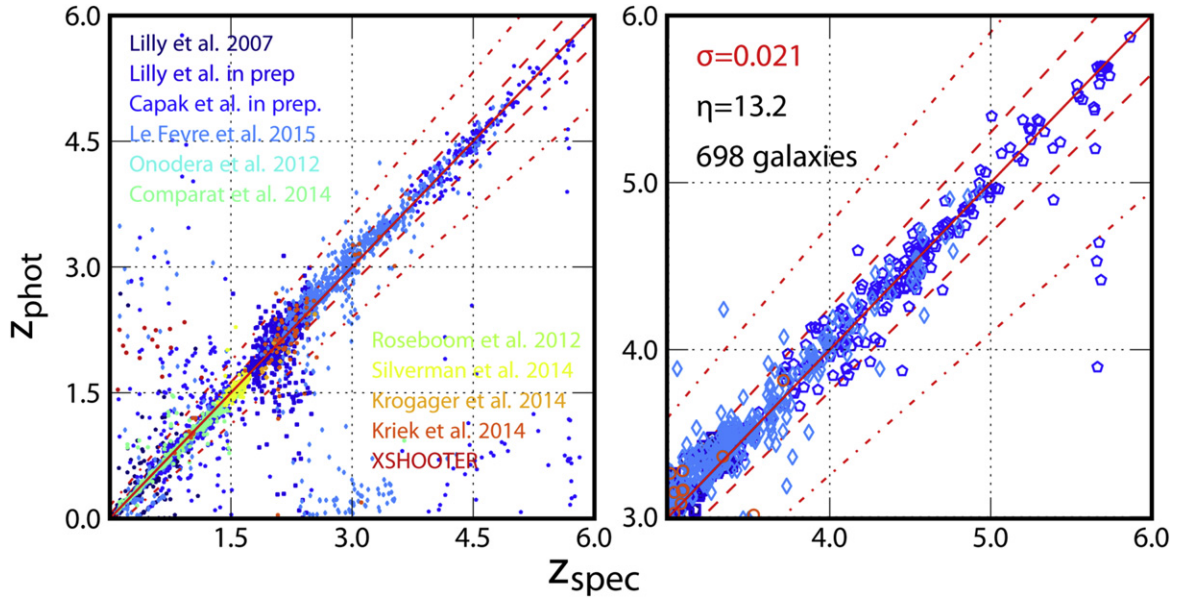
Figure 12. Left: comparison between photometric and spectroscopic redshifts for the different samples summarized in Table 5. Right: a magnified view of the high-redshift region. The number of galaxies, accuracy \sigma , and numbers of catastrophic failures \eta and \eta_{\text{lim}} are computed from the zCOSMOS-faint, VUDS, DEIMOS, FMOS, and MOSDEF spectroscopic surveys taken together, keeping only non-flagged galaxies with a spectroscopic redshift greater than 2.9. The dashed and dashed-dot lines show z_p = z_s \pm 0.05(1 + z_s) and z_p = z_s \pm 0.15(1 + z_s) , respectively. Note that the given value for the precision and the percentage of catastrophic failures strongly depend on the spectroscopic sample. These values are detailed in Table 5.
