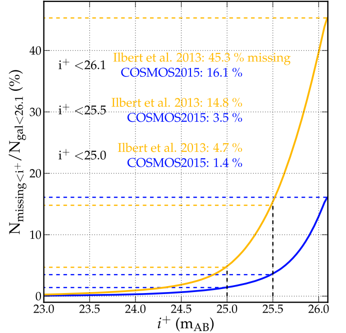
Figure 8. Cumulative distribution of the number of galaxies over the total number of galaxies in a magnitude-limited sample ( i^+ < 26.1 ) as a function of magnitude in the i^+ band from Capak et al. (2007) which are not recovered in Ilbert et al. (2013; orange line) and this catalog (blue line).
