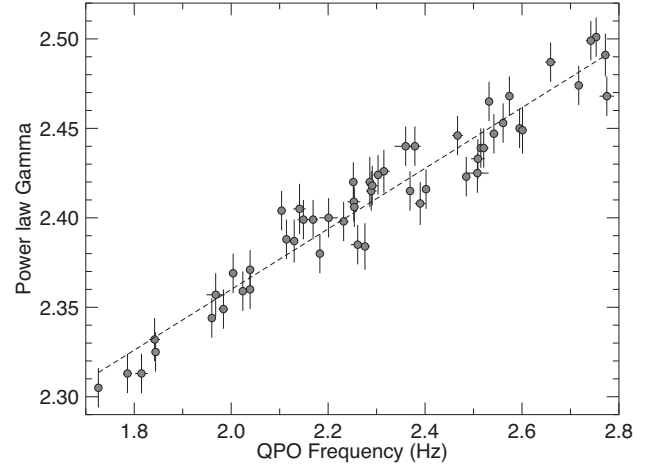
Figure 7. Correlation between power-law spectral index \Gamma and QPO centroid frequency \nu_{\text{QPO}} . The line is the best-fitting linear correlation. The segments in which SXT data were not available are not included.
