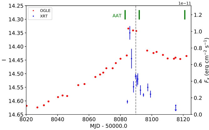
Fig. 3. Magnified view of the December 2017 outburst seen by OGLE (red points). Superimposed are the 0.3–8 keV fluxes from the Swift /XRT monitoring of AX J0049.4–7323 (blue points), and the times of the AAT observations (green bars). The grey vertical dashed line shows the expected time of the peak of the optical outburst calculated with the ephemeris of Schmidtke et al. (2013).
