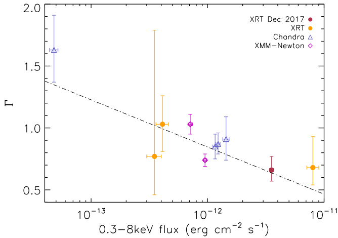
Fig. 7. Photon index ( \Gamma ) as a function of the absorbed flux. Errors are quoted at the 1\sigma confidence level. The plotted values correspond to those listed in Table 3 of Ducci et al. (2018; yellow circles, blue triangles, magenta diamonds) and Table 2 of this paper (red circle).
