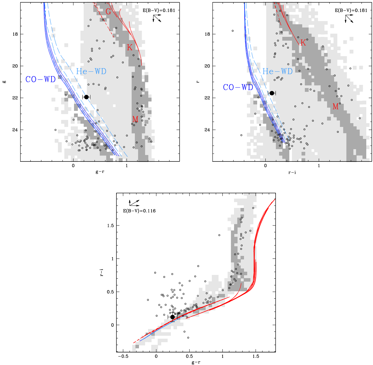
Figure 2. Observed CM (top row) and CC (bottom row) diagrams for all the stars in a \sim 2.0 \text{ arcmin} \times 5.5 \text{ arcmin} sky region around the PSR J0614–3329 position (filled black circles). The candidate companion star to the pulsar is marked by the black filled circle. Stellar sequences simulated from the Besançon models for different values of distance are shown in light and dark grey. In the CM diagrams the dark grey regions correspond to distance values within \pm 20 percent the assumed pulsar distance (see Table 5), whereas in the CC diagram they correspond to magnitudes within \pm 0.05 the r -band magnitude of the pulsar candidate companion star. Theoretical evolutionary tracks for both He WDs ( 0.2, 0.25, 0.35 M_{\odot} ; light blue dashed lines) and low-mass CO WDs ( 0.35, 0.4, 0.45 M_{\odot} ; dark blue solid lines) are represented, computed from the models of Panei et al. (2007) for an age up to 4.8 Gyr and for the nominal values of the MSP distance. Masses increase from right to left. Evolutionary tracks for MS stars for both Z = 0.02 (red solid lines) and Z = 0.0001 (red dashed lines) are also shown for different mass ranges ( 0.5\text{--}1 M_{\odot} , with steps of 0.1 M_{\odot} ) and for the nominal MSP distance. Masses decrease from top to bottom. Only in this case we assumed a distance value half of that obtained from the DM (see discussion in Ransom et al. 2011). Both the simulated stellar sequences from the Besançon models and the WD and MS evolutionary tracks were plotted assuming a null reddening. Reddening vectors are shown on the top of each panel. The lengths of the vectors correspond to the E(B-V) estimated from the hydrogen column density inferred from the fits to the MSP X-ray spectrum. We used the extinction coefficients of Fitzpatrick (1999).
