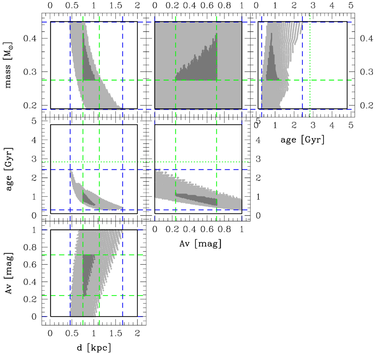
Figure 5. Pair combinations of the four parameters which we used to fit the observed magnitudes and colours of the candidate companion star to PSR J0614–3329 with model evolutionary tracks (Panei et al. 2007). This plot refers to the case of an He WD. The thick black lines mark the investigated region in each plane of the parameter space. The light grey regions mark, for each pair of parameters, the allowed parameter configurations which reproduce the observed optical properties of the candidate companion stars (magnitudes, colours). The extreme of these regions projected on each axis are marked by the blue lines, while the green dashed lines mark the parameter range constrained by the radio and X-ray measurements. Although the radio/X-ray constraints of each parameter pair seem to be more stringent than the optical ones, imposing that all conditions are simultaneously satisfied shrinks the allowed parameter configurations to the dark grey regions. The dotted green line corresponds to the pulsar spin-down age.
