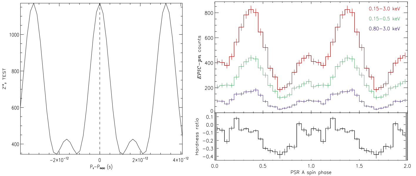
Figure 1. Left: result of the pulsar spin period search trials around PSR A’s radio ephemeris solution. The most significant X-ray pulsed detection corresponds to a Z^2_{\text{TEST}} value of \sim 1200 and is precisely aligned (within \sim 10^{-13} s) with the radio period indicated by the dashed vertical line. Top right: background-subtracted light curve of PSR A for the energy band 0.15–3.0 keV (in red) and two sub-bands at low (0.15–0.5 keV, green) and high (0.8–3.0 keV, blue) energies, resulting from epoch folding of all available EPIC-pn data (2006+2011). Bottom right: phase-resolved hardness ratio between the hard (0.8–3.0 keV) and soft (0.15–0.3 keV) energy bands.
