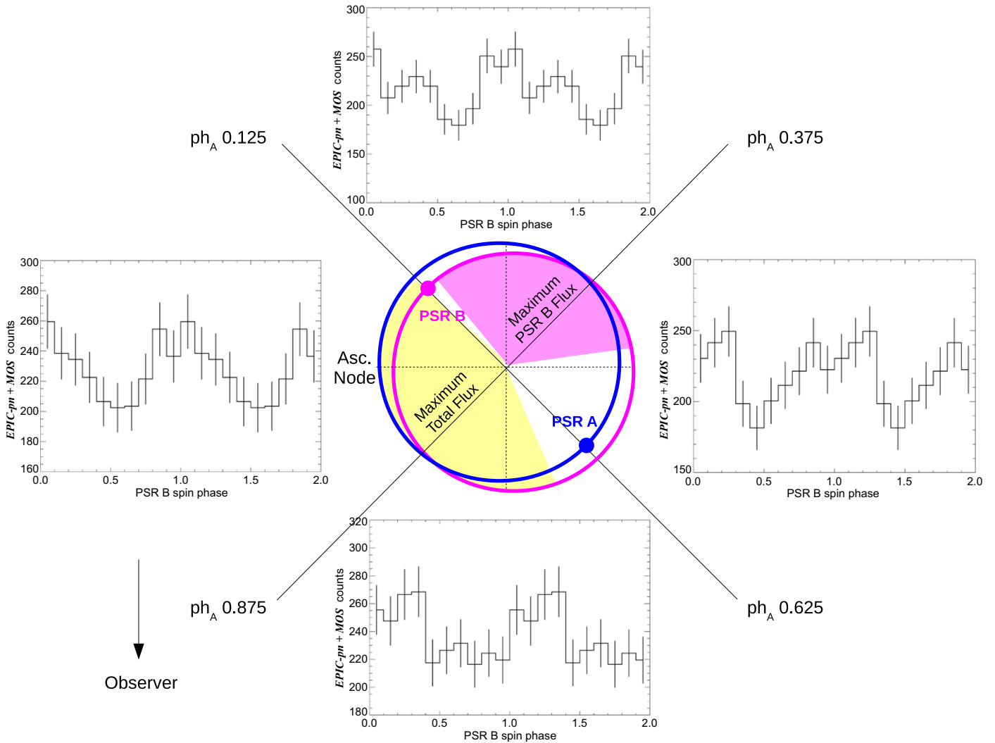
Figure 4. Central panel: scheme of the orbital configuration of PSR J0737–3039 in 2011 subdivided into four orbital phase intervals containing conjunctions ([0.125, 0.375]–[0.625, 0.875]) and quadratures ([0.875, 0.125]–[0.375, 0.625]). The yellow shaded region corresponds to the maximum of the total X-ray flux from the system (see Section 5 and Figure 5), while the pink area indicates the maximum of the PSR B pulsed flux (both shaded regions highlight the orbital phase intervals where PSR B is passing). The ph_A label in the figure highlights that phase 0 refers to the PSR A ascending node. The four plots displayed around the scheme show the PSR B (background-subtracted) pulse profile obtained by folding the 2011 EPIC-MOS and EPIC-pn counts belonging to the above mentioned orbital phases for the 0.15–3.0 keV energy band (the pulsed profiles are referred to as the orbital phase intervals where PSR B is passing).
