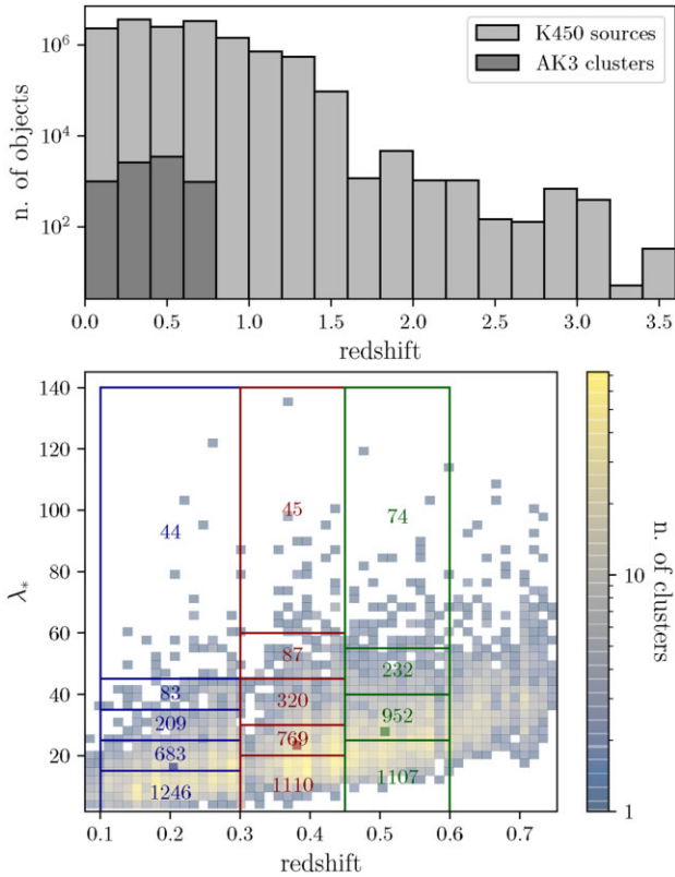
Figure 1. Top panel: Redshift distributions of AK3 clusters (dark grey) and K450 galaxies (light grey). Bottom panel: AK3 clusters in the redshift-richness plane with \text{SNR} \geq 3.5 . Coloured rectangles correspond to the redshift-richness bins used in the following analysis (see Section 3.4); the number of clusters enclosed in each bin is displayed. Single coloured squares show the mean values in each redshift bin computed as in equation (17).
