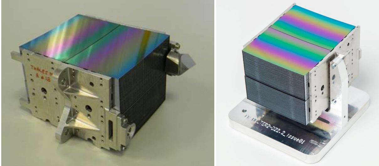
Figure 6 – Photos of two of the four mirror modules, differentiated by their bracket type, produced during the production run in 2017. The left image shows a mirror module prepared for the AIT activities led by TAS Switzerland, the right photo shows a Media Lario module. Each mirror module consists of 2 pairs, called an XOUs, of a primary and a secondary mirror stack.
