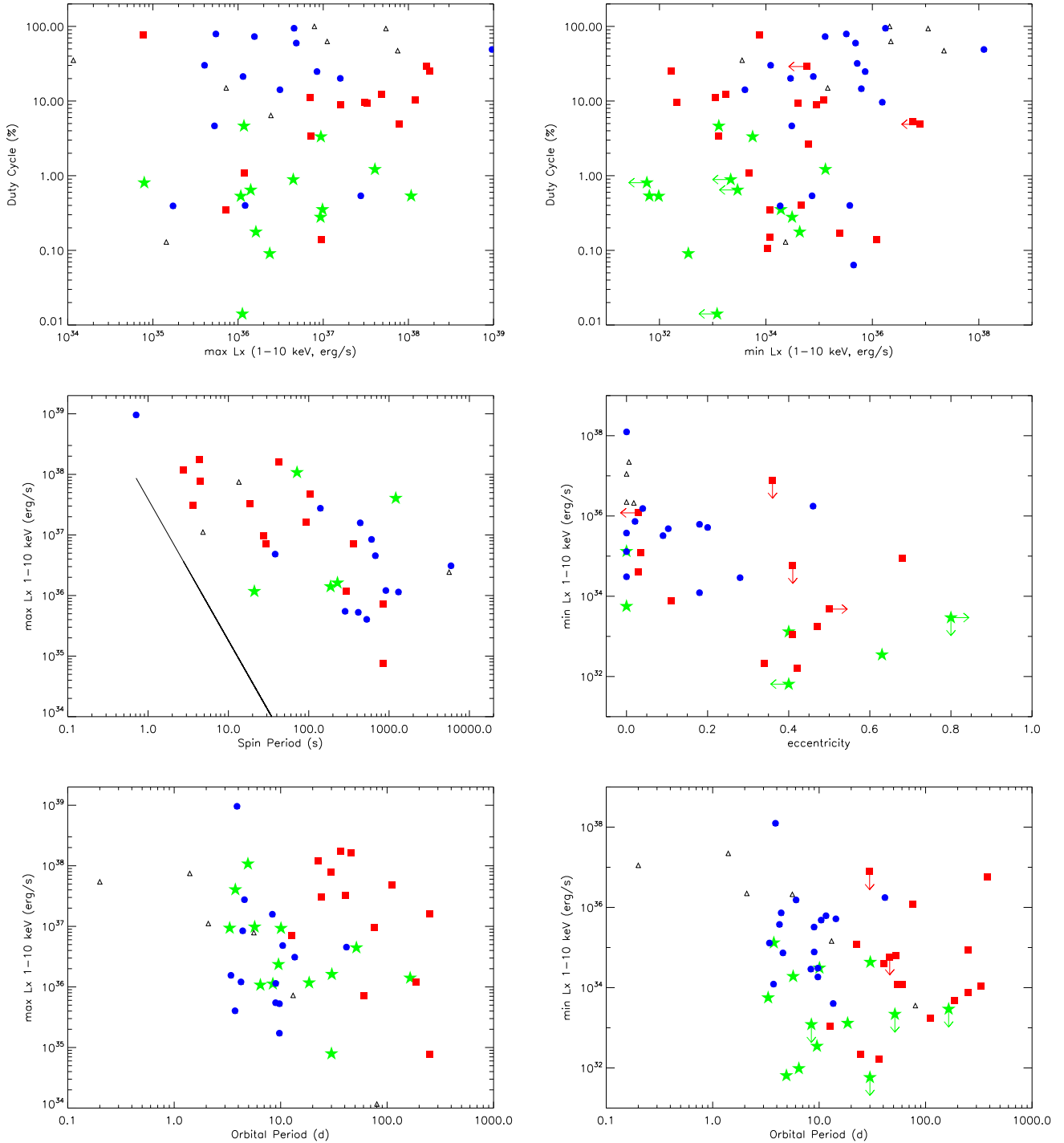
Figure 15. Properties of the sources in our sample, presented in Tables 1 and 2. The meaning of the symbols is the same as in Figs. 11 and 12. In the plot of the maximum luminosity (1–10 keV) against the spin period, the minimum luminosity before the on-set of the propeller effect is drawn (solid line), following equation (3) (assuming an NS magnetic field of 10^{12} G and \xi = 1 ).
