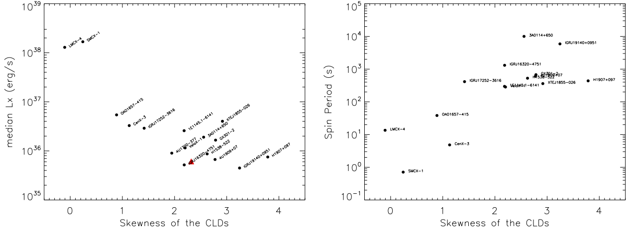
Figure 7. Median luminosity (18–50 keV; left-hand panel) and pulsar spin period (right-hand panel) versus the skewness of the CLDs, for giant and supergiant HMXBs with DC_{18-50\text{ keV}} larger than 1 per cent. The red triangle on the left-hand panel indicates the position of the SgB[e] binary IGR J16318–4848 (see Section 5.1.5).
