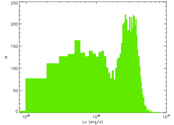
Figure 8. Cyg X-1 luminosity distribution (18–50 keV). Here, the bimodality is more evident than in the correspondent CLD shown in Fig. 4.
