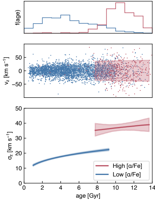
Fig. 9. Vertical ( \sigma_z ) velocity dispersion as a function of age. Middle panel: best-fit models for the AVR of the low- and high- [\text{Mg}/\text{Fe}] selection in age- v_z space, compared with the data used in the fit. Lower panel: AVRs themselves, and upper panel: age distribution of the [\alpha/\text{Fe}] selected populations. Blue and red lines represent the best fit power-law models for stars in the low- and high- \alpha sequence, respectively. The coloured bands in the lower panel show the 5th to 95th percentile credible intervals of the inferred \sigma_z -age relation. The AVR for each population is only shown in the range of the 0.05 and 0.95 quantile of its ages.
