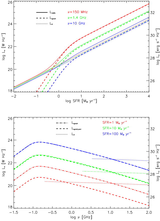
Figure 4. Top panel: synchrotron (dashed, including the suppression for small SFR after Equation (9)), free-free (dotted), and total radio (solid) luminosity from an SFG as a function of the SFR for three different frequencies \nu \approx 0.15 (red), 1.4 (green), and 10 GHz (blue). Bottom panel: synchrotron (dot-dashed lines refer to Equation (7), while dashed lines include the suppression for small SFR after Equation (9); curves are distinguishable only for the smaller SFR) and free-free (dotted) luminosity as a function of frequency for three different values of the SFR \dot{M}_* \approx 1 (red), 10 (green), and 100 M_\odot \text{yr}^{-1} (blue).
