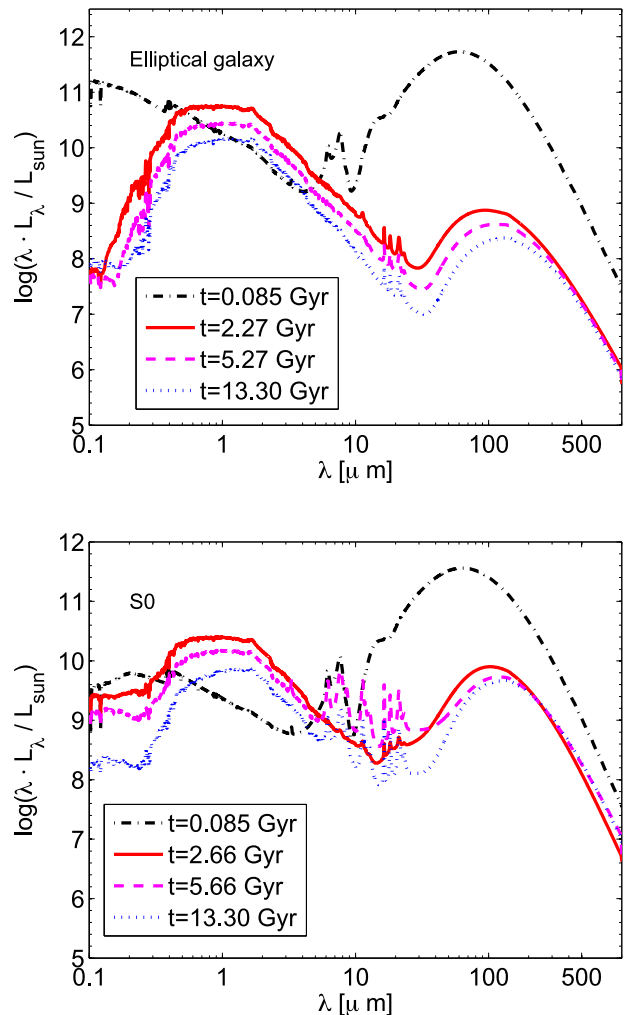
Figure 3. Time evolution of the SED of modelled galaxies of early morphological types – upper panel: elliptical; lower panel: S0 – of M = 10^{11} M_{\odot} for four significant ages, as the legend indicates.
