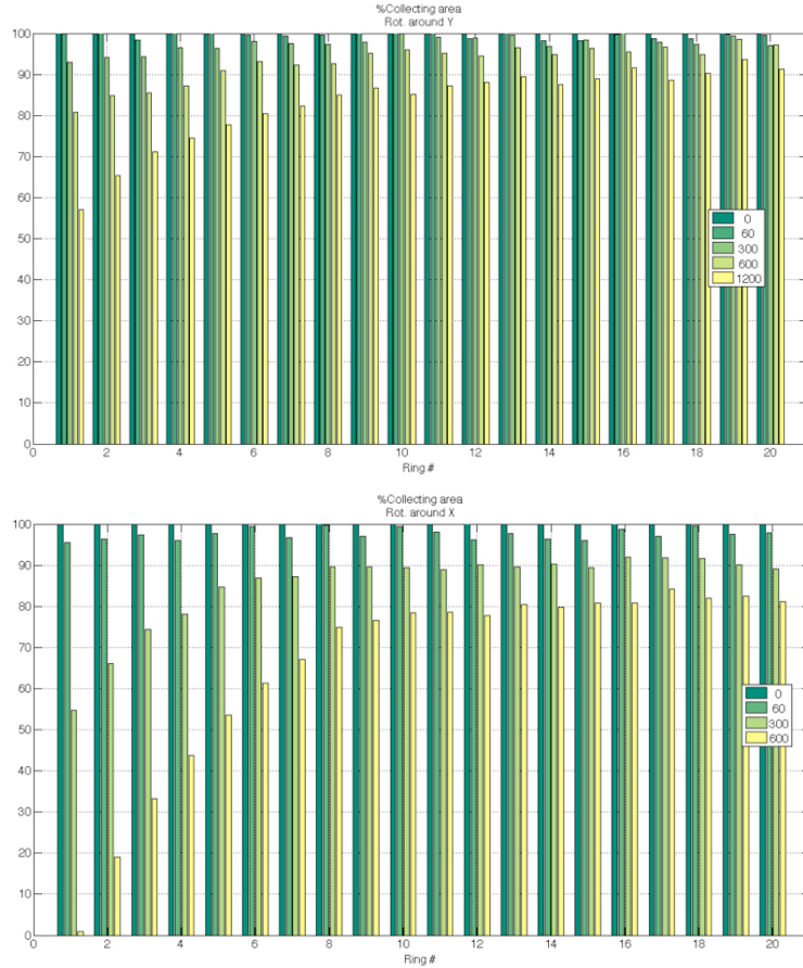
Figure 10. Percent of residual collecting area with respect to the on-axis configuration for different rotation amplitudes (0 , 60, 300, 600, and 1200 arcsec). Top: rotation around y -axis. Bottom: rotation around x -axis.
