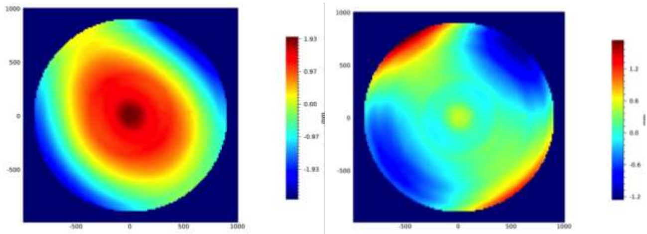
Figure 4 – Replicated glass substrate shape error residuals compared to the theoretical design (left) and the theoretical mirror shape, leaving the RoC as a free parameter (right).
