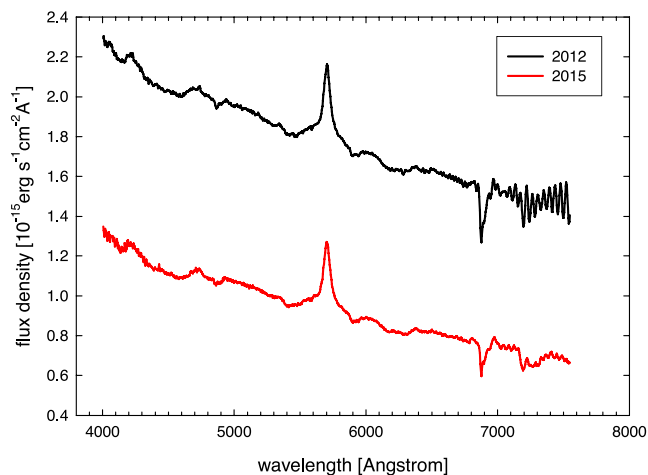
Figure 9. Averaged spectra of CTA 102 during the 2012 and 2015 observing seasons. Absorption features longwards of \lambda 6800 Å are of telluric origin.
