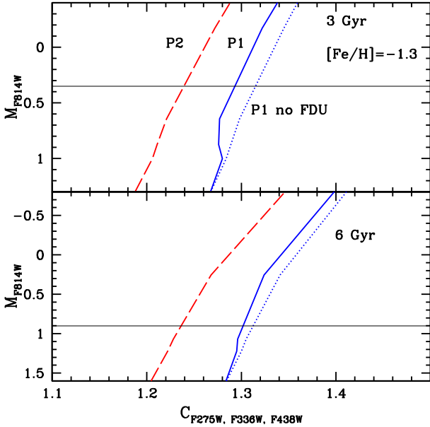
Figure 2. P1 (solid lines) and P2 (dashed lines) RGBs (at [\text{Fe/H}] = -1.30 ) in the M_{\text{F814W}} - C_{\text{F275W, F336W, F438W}} diagram for ages equal to 3 (upper panel) and 6 (lower panel) Gyr, \Delta[\text{N/Fe}]_{\text{ini}} = 0.8 , accounting for the effect of FDU on the spectral energy distributions. The dotted lines display P1 RGBs calculated without considering the variation of N (and C) due to the FDU. The horizontal thin lines mark the level corresponding to two magnitudes above the main-sequence turn-off, where the width of the RGB is taken in the chromosome maps (see the text for details).
