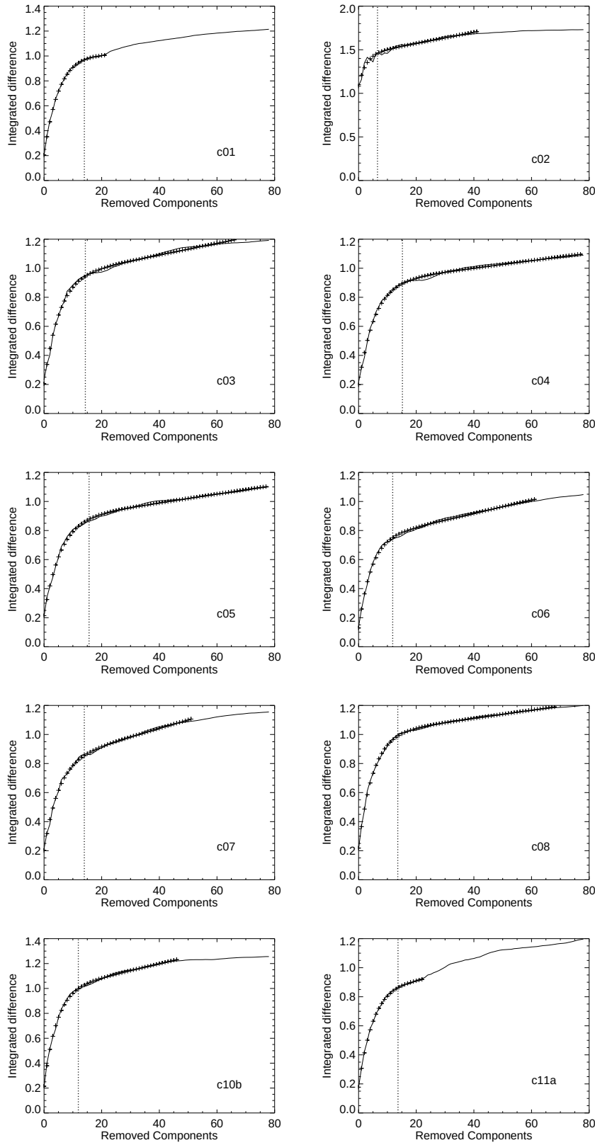
Fig. 2 Integrated difference of the variance at different component removed (black line) for Campaign 1 to 11a, in which the best fit (cross points) and the component at 3\sigma (vertical dashed line) are shown.
