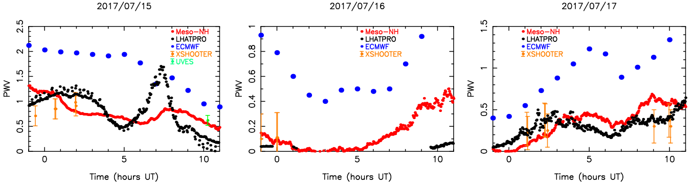
Figure 6. Time evolution of PWV values over three nights centered around the extremely low PWV event of 2017/07/17. Black dots correspond to LHATPRO measurements, red dots correspond to the Meso-NH forecast (2-minutes sampling time), the blue dots corresponds to the ECMWF forecast (1-hour sampling time), the orange dots corresponds to X-SHOOTER measurements and green dots corresponds to UVES measurements. According to Table 6, we estimate the Meso-NH model error to be around 0.25 mm.
