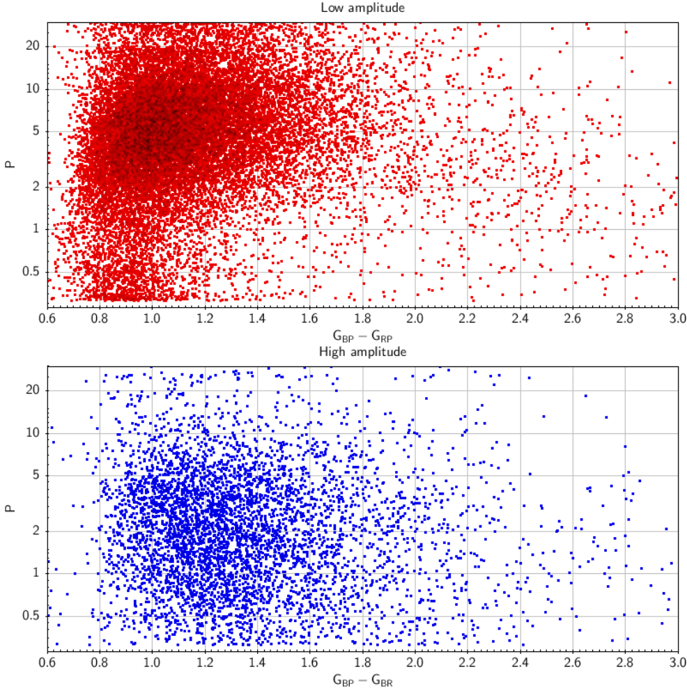
Fig. 9. Period-colour diagrams for the low-amplitude population ( \max A_{\text{fit}} \leq 0.04 , upper panel ), and for the high-amplitude population \max A_{\text{fit}} > 0.04 , ( lower panel ). P is given in day units.
