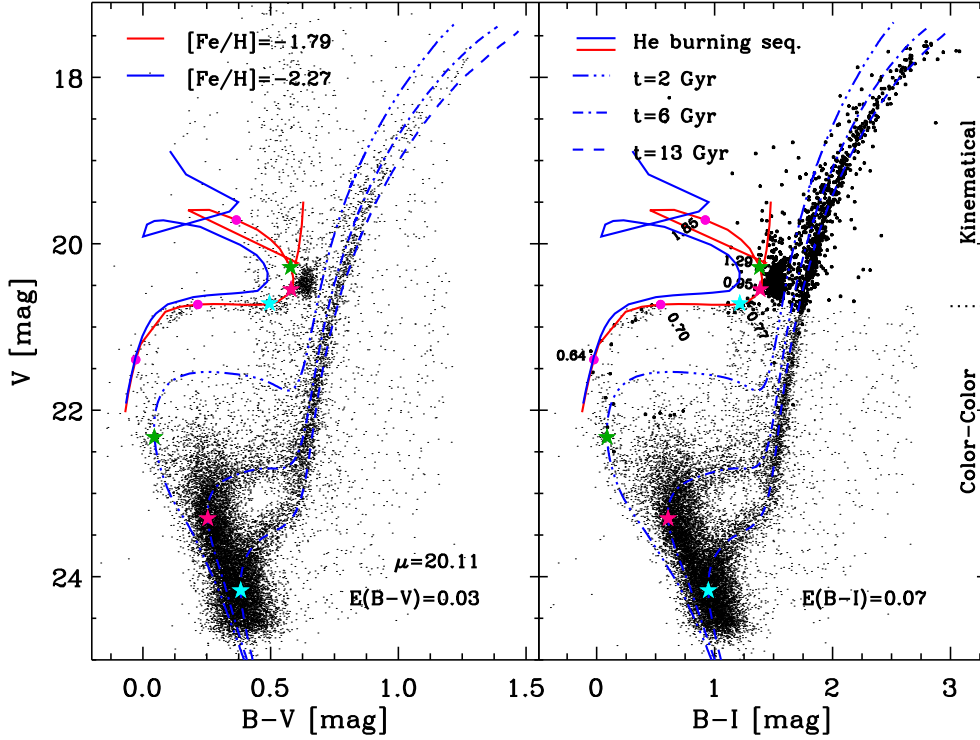
Fig. 1. Left – Comparison in the V , B - V CMD between candidate Carina stars selected on the basis of the U - V , B - I color-color plane (Bono et al. 2010a) and isochrones computed adopting a scaled-solar chemical composition ( [\text{Fe}/\text{H}] = -1.79 ). The ages range from 2 (dashed-dotted-dotted) to 13 (dashed) Gyr. The solid blue and red lines show the predicted He burning sequences for two different iron abundances. The adopted true distance modulus and reddening are also labelled. Right – same as the left, but for the V , B - I CMD. The 1379 stars with visual magnitudes brighter than 20.75 were selected according to kinematic properties (Fabrizio et al. 2011). The labels along the metal-poor He burning sequence display selected mass values (see text for details).
