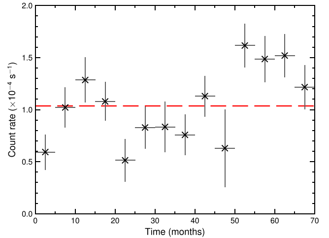
Figure 2. Hard X-ray (14–195 keV) light curve of NGC 6240 from the Swift /BAT 70-month survey (2004 December to 2010 September) in time bins of 5 months, commensurate with the separation between the last three NuSTAR observations. The source is clearly variable around the average (red dashed line), and significant flux changes can occur on time-scales of about 1 yr.
