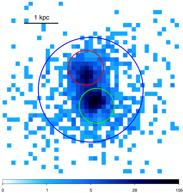
Figure 1. Chandra image of the central ( 10 \times 10 arcsec 2 ) region of NGC 6240 in the 5–7.5 keV band (rest frame), obtained by combining the ACIS-S observations of 2001 July (ObsID 1590) and 2011 May (ObsID 12713). Subpixel resolution by a factor of 2 is adopted, so one pixel in this figure has a physical size of 126 pc. The regions employed in the spatially resolved spectral analysis are also shown: northern nucleus (red), southern nucleus (green) and diffuse Fe K emission (blue).
