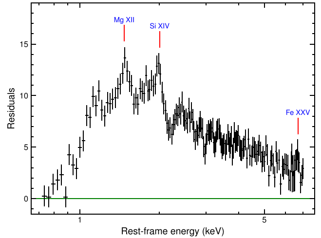
Figure 7. Residuals (in units of \sigma ) in the Chandra spectrum of the whole galaxy (rebinned by a factor of 2 for clarity) with respect to a model consisting of the spatially resolved shock, reflected continuum and nuclear components plus the large-scale emission from the cold and warm gas phases. The shape closely resembles a thermal spectrum with an absorption cut-off at lower energies. Three major features can be clearly identified from Mg XII, Si XIV and Fe XXV, which mainly originate from the shock-heated gas (compare with Fig. 4).
