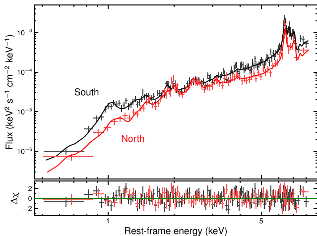
Figure 5. Resolved Chandra spectra of the southern (black) and northern (red) nucleus of NGC 6240, with best-fitting models and relative residuals (in units of \sigma ). Even the simple visual inspection reveals that all of the thermal components are inherently clumpy and that their temperature and obscuration is locally variable. Note that some additional Ni K \alpha emission at 7.47 keV might be present in both nuclei.
