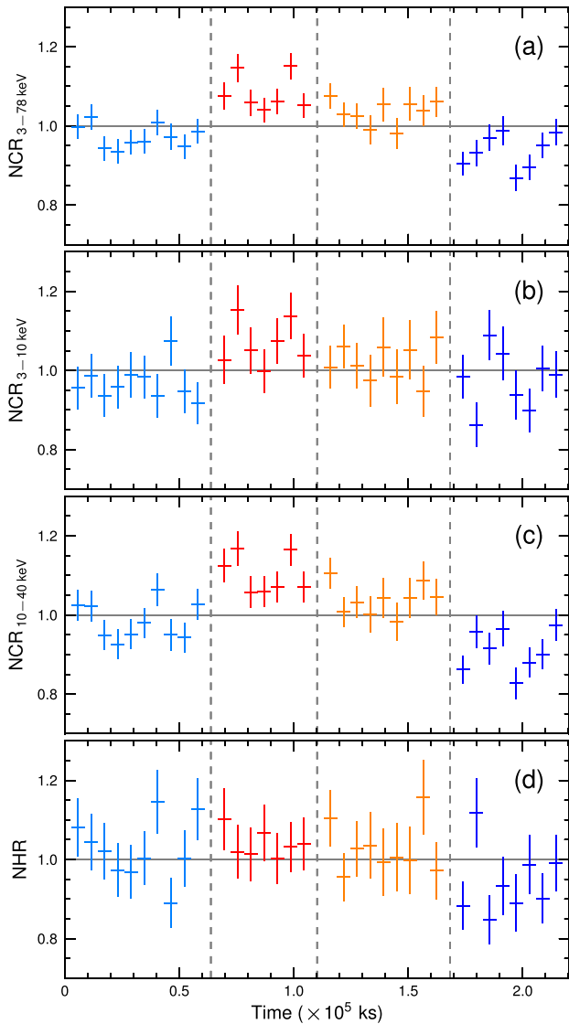
Figure 3. From top to bottom: normalized count rates in the (a) 3–78, (b) 3–10, (c) 10–40 keV bands and (d) normalized 10–40/3–10 keV hardness ratio for the four NuSTAR observations. The background-subtracted light curves from both modules were added together, after the standard corrections for dead time, PSF and vignetting losses. The horizontal scale portrays the total elapsed time, with the gaps between the observations removed.
