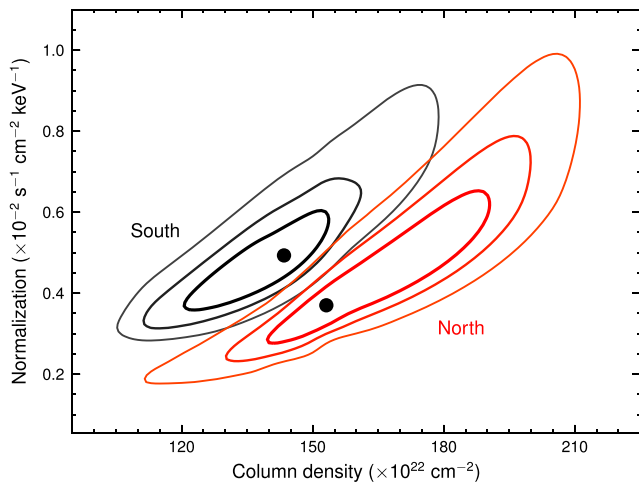
Figure 6. Confidence contours at the 68, 90 and 99 per cent levels in the primary continuum normalization versus column density plane for both nuclei. Despite the mild degeneracy between these quantities, the southern nucleus is generally confirmed to be the brighter and less obscured one. For larger differences between the column density values, however, solutions of equal intrinsic luminosity are still completely allowed.
