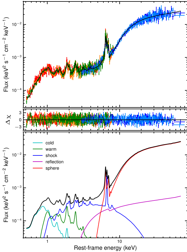
Figure 4. Top panel: average XMM-Newton (red for pn, orange for MOS), Chandra (green), and NuSTAR spectra (light and deep blue for FPMA and FPMB) of NGC 6240, corrected for cross-normalization. Best-fitting Model B is superimposed (black curve). Mid panel: residuals in units of \sigma . Bottom panel: contribution of the different spectral components, convolved with the Chandra ACIS-S response up to 8 keV, and with the NuSTAR one beyond.
