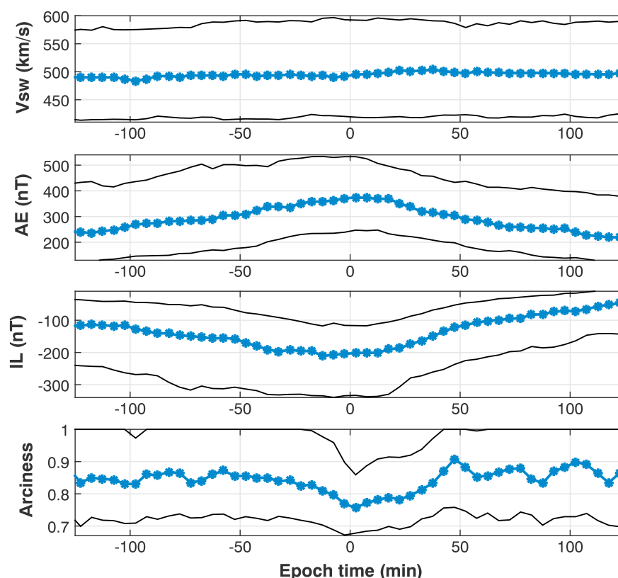
Figure 4. (first panel) Solar wind speed (km/s), (second panel) AE index (nT), (third panel) IL index (nT), and (fourth panel) arciness index as a function of epoch time in minutes. The blue curves are the median values and the black curves are 25th and 75th percentiles, respectively. Zero epoch time is the time when pulsating aurora becomes the dominant aurora type in a camera FOV. The \pm 2 h from the zero epoch time is shown because it captures the most dramatic changes.
