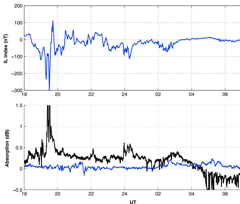
Figure 2. (top) Local electrojet ( IL ) index (nT) and (bottom) cosmic radio noise absorption from Ivalo (black) and Longyearbyen (blue) station for the sample event on 30–31 December 2003.
