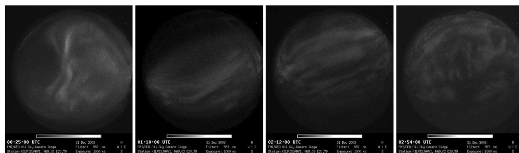
Figure 3. KIL auroral images of diffuse nonpulsating aurora (00:25 UT) to pulsating arcs (01:10 UT), large elongated pulsating patches (02:12 UT), and small pulsating features (02:54 UT). Image brightness has been enhanced for better visibility of the emission structures of interest.
