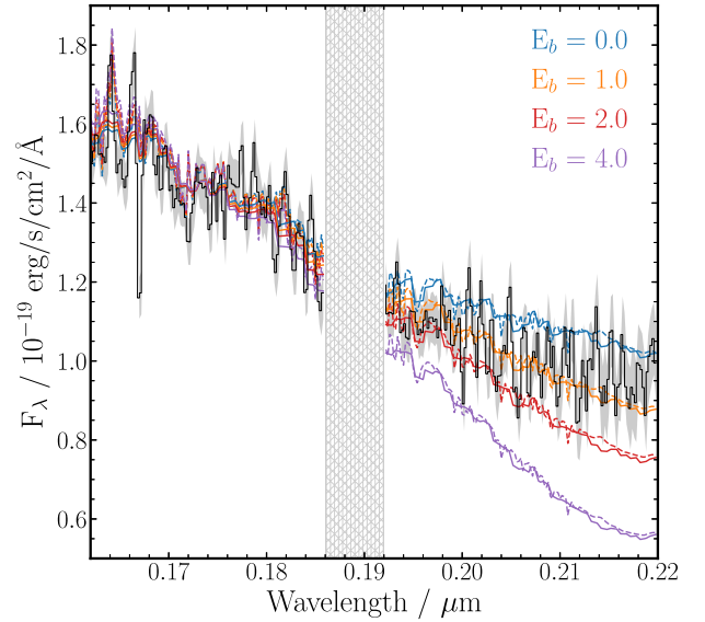
Figure 12. Investigating evidence for excess attenuation at 2175 Å from a composite of 122 VANDELS spectra at 3.0 \leq z \leq 3.5 ( \langle z \rangle = 3.288 ). The grey spectrum is the composite VANDELS spectrum with the grey shaded region representing the \pm 1\sigma error. The hatched region around \lambda \sim 0.19 \mu\text{m} masks the C III \lambda 1909 emission line. The solid and dashed coloured curves show, respectively, the FiBY-BPASSv2-300bin and S99-v00-z008 templates reddened using the Noll et al. (2009) attenuation curve assuming four values of the 2175 Å bump strength ( E_b ; see the text for details). For each value of E_b the templates have been attenuated with A_V = 0.8 assuming the Calzetti A_V – M_* relation at the median mass of the galaxies contributing to the stack ( \log(M_*/M_\odot) = 9.71 ; see Fig. 9).
