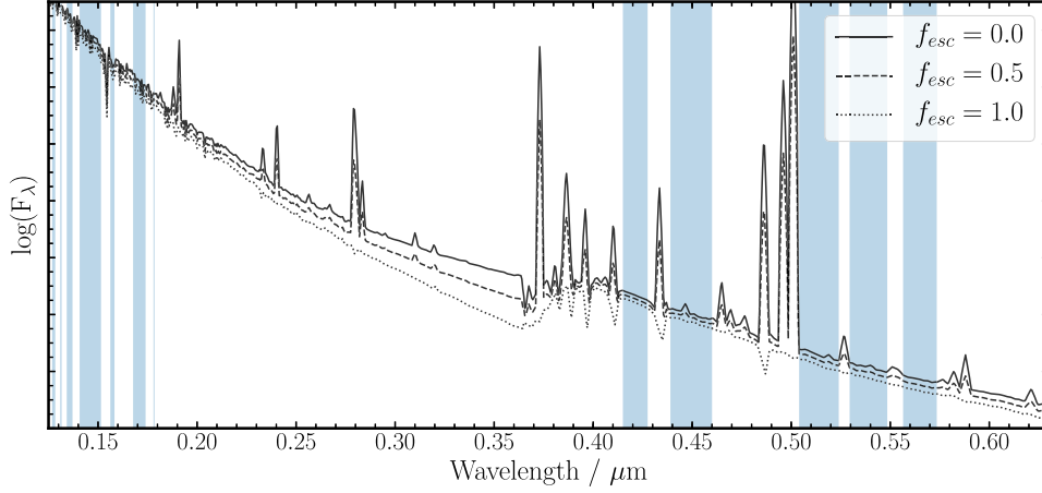
Figure 5. The intrinsic FiBY-BPASSv2-300bin SED across the wavelength region 0.125 \mu\text{m} < \lambda < 0.63 \mu\text{m} assuming different values for the escape fraction of ionizing photons ( f_{\text{esc}} ). It can be seen that some wavelength regions are extremely sensitive to the nebular spectrum and therefore unsuitable to use when fitting the attenuation curve (see the text for details). The blue shaded areas show the wavelength regions we defined as suitable to use. These wavelength pixels satisfied the following criteria: (i) a maximum nebular contribution of 10 per cent; (ii) free from any strong stellar absorption/emission features.
