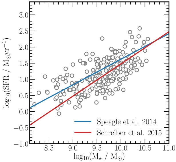
Figure 1. The position of our VANDELS sample in the M_* –SFR plane. Masses and star formation rates were derived using the SED fitting code LEPHARE (see the text for details). For comparison, the blue and red lines show two independent determinations of the main sequence of star formation at z = 3.5 from Speagle et al. (2014) and Schreiber et al. (2015), respectively. It can be seen that the galaxies in our sample are consistent with being typical star-forming galaxies at z = 3.5 .
