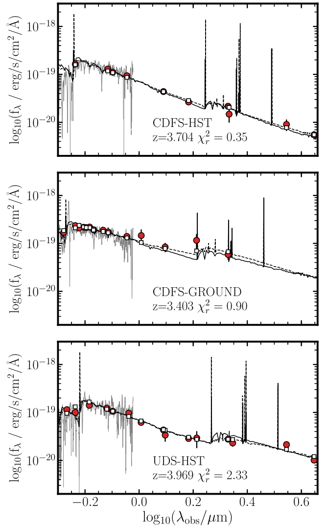
Figure 2. The UV-to-optical SEDs for three galaxies in our sample. In each panel, the red circular data points show the observed photometry while black solid/dashed spectra show the best-fitting LePhare / EAZY templates, respectively. The open squares show the synthetic photometry of the best-fitting EAZY template through the observed filters. The grey spectra at \lambda \approx 0.5-1.0 \mu\text{m} ( \log(\lambda/\mu\text{m}) \approx -0.3-0.0 ) are overlays of the observed VANDELS spectra, which we used to accurately determine the redshift of the galaxies.
