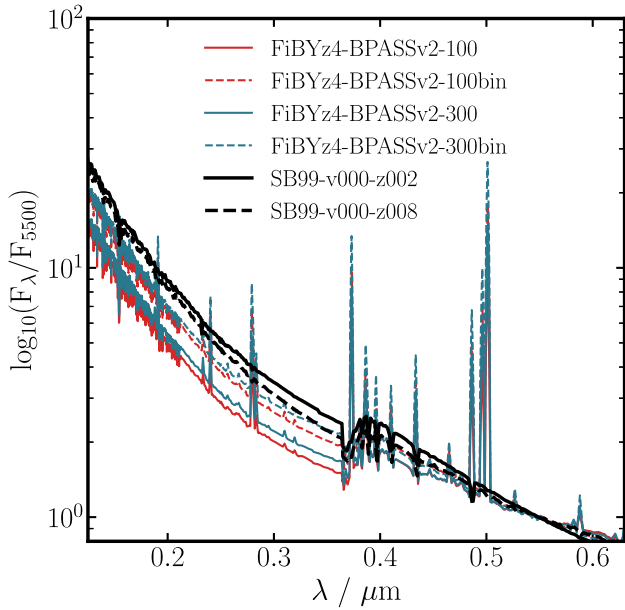
Figure 4. The six template spectra used as the intrinsic (dust-free) SED shapes when deriving the dust attenuation curve. The red lines show stacked synthetic spectra of FiBY simulated galaxies at z = 4 (see text for details) for the FiBY-BPASSv2-100 model (solid) and FiBY-BPASSv2-100bin model (dashed) respectively. The blue lines show the same for the BPASSv2 models with an upper IMF cutoff of 300M_{\odot} (FiBY-BPASSv2-300, FiBY-BPASSv2-300bin). Finally, the solid and dashed black lines show the S99-v00-z002 and S99-v00-z008 constant star-formation rate Starburst99 models, both with age 100 Myr, respectively. All spectra are normalized at 0.55 \mu\text{m} .
