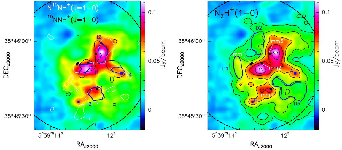
Figure 4. Left-hand panel: The colours are the averaged emission of \text{N}_2\text{H}^+(1-0) . The black contours are the 5\sigma levels of ^{15}\text{NNH}^+(1-0) averaged emission and the white contours are the 5\sigma levels of ^{15}\text{NH}^+(1-0) averaged emission: in blue the intersection of the black and white contours (I1, I2, I3, and I4). Right-hand panel: the same as Fig. 2. The blue contours define three different zones D1, D2, and D3, in the diffuse \text{N}_2\text{H}^+ envelope surrounding the dense condensations identified in the left-hand panel and in Fig. 3. In both panels, the black and blue squares indicate the positions of the continuum sources and the \text{N}_2\text{H}^+ peak positions (A and B), respectively, as in Fig. 2. The dashed circle represents the NOEMA field of view.
