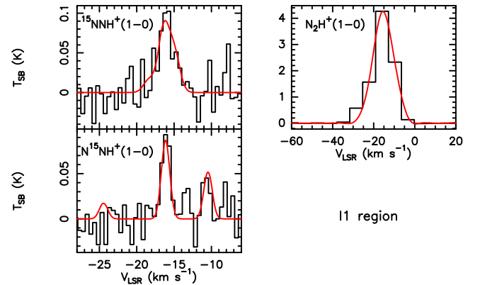
Figure 5. Example of spectra extracted from the region I1 (see left-hand panel of Fig. 4) in all the detected transitions: ^{15}\text{NNH}^+(1-0) (top left), ^{15}\text{NH}^+(1-0) (bottom left), and \text{N}_2\text{H}^+(1-0) (top right). For each spectrum the x-axis represents the systemic velocity of the source. The y-axis shows the intensity in synthesized beam temperature units. The red curves are the best fits obtained with MADCUBA (from the method described in Section 3.3). Spectra extracted from the other intersecting regions (I2–I4) are shown in Appendix A2.
