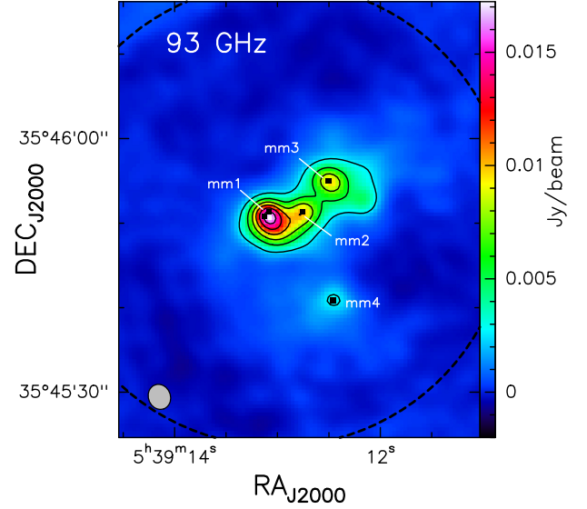
Figure 1. 93 GHz continuum emission obtained with IRAM NOEMA. The first contour level is the 15 per cent of the maximum value of the map, which corresponds to \sim 17 \text{ mJy beam}^{-1} . The other contour levels are the 30 per cent, 45 per cent, 60 per cent, 75 per cent, and 90 per cent of the maximum value, respectively. The black squares indicate the position of mm1a, mm1b, mm2, mm3, and mm4 as given in the text and in Table 1. The dashed circle represents the NOEMA field of view and the synthesized beam is the ellipse indicated in the lower left corner.
