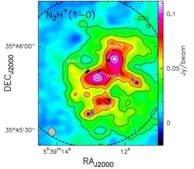
Figure 2. Averaged map of \text{N}_2\text{H}^+(1-0) at 93.1734 GHz (velocity range between -34.6 and -0.1 \text{ km s}^{-1} ) obtained from the Windex correlator. The contour levels are 4, 7, 10, 13, 16, and 18 times the 1\sigma rms of the map, equal to \sim 6 \text{ mJy beam}^{-1} . The black squares indicate the position of mm1a, mm1b, mm2, mm3, and mm4 as given in the text and in Table 1. The blue squares correspond to the \text{N}_2\text{H}^+(1-0) emission peaks, A and B, described in the text. The dashed circle represents the NOEMA field of view and the synthesized beam is the ellipse indicated in the lower left corner.
