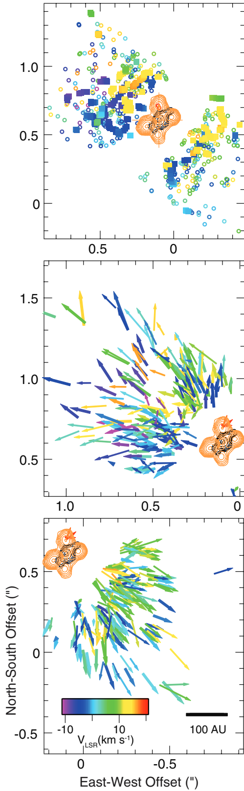
Figure 1: Maser kinematics in Source I. Left Panel) Top: SiO v=0 and H 2 O masers ( open circles and squares , respectively – [5]), velocity-integrated SiO v=1 masers ( red contours – [4]), and 7 mm continuum ( black contours – [11]), as mapped with the VLA. Middle: expanded view of SiO v=0 maser proper motions in the northeastern lobe of Source I. Bottom: expanded view of the southwest lobe. Colors denote maser V_{\text{LSR}} as indicated in the wedge on the bottom left corner of the bottom panel. Right Panel) Combined (velocity-integrated) SiO v=1 and v=2 maser emission distribution ( red-tone image ) observed with the VLBA [8], and 7 mm continuum ( color map ) imaged with the VLA [11].
