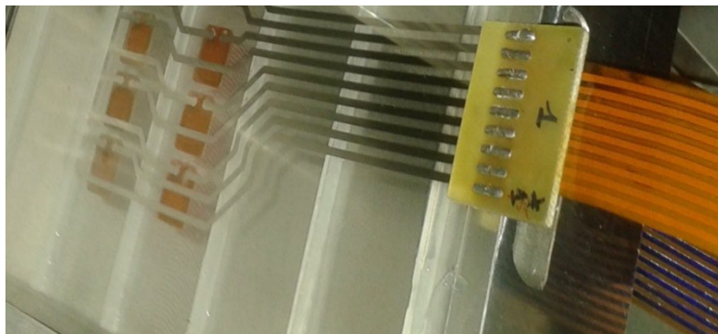
Figure 5. Ad-hoc connector and flex cable attached to the glass.
