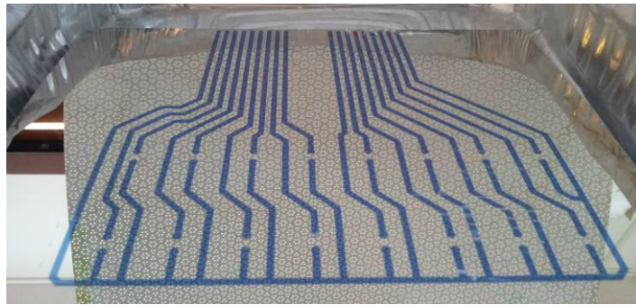
Figure 2. Electric tracks deposited on the back of a curved thin glass. They are still protected by a photoresist film.
