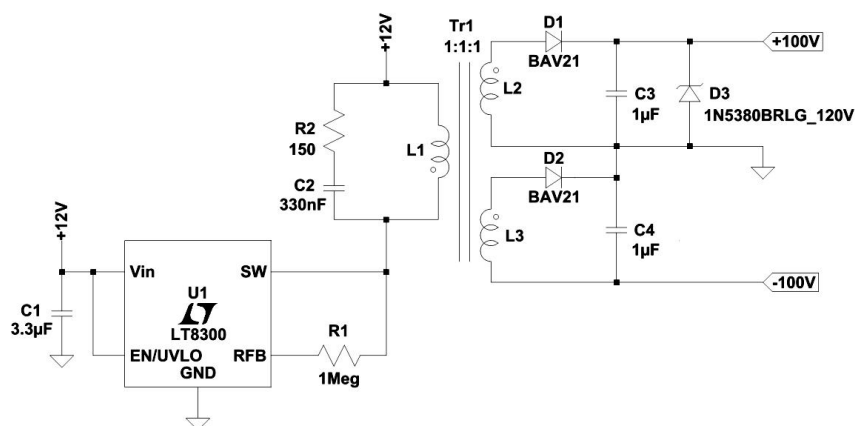
Figure 11. High voltage DC-DC converter schematic.
