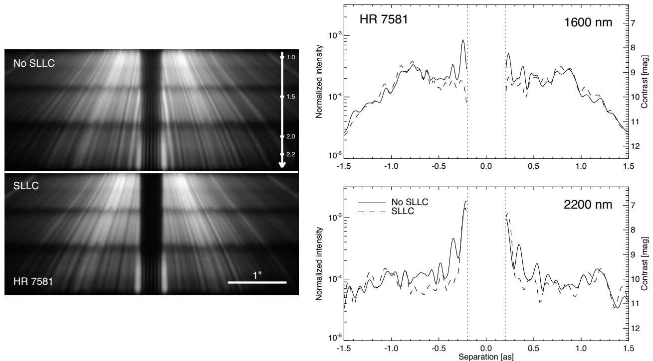
Figure 8. Left : On-sky IRDIS/LSS data acquired on the star HR 7581 without (top) and with the SLLC (bottom). The wavelength scale (in micron) is indicated with the downward white arrow. The total spectral range is 0.95\text{--}2.3\ \mu\text{m} , and the spatial extension is 2.5'' . The horizontal dark lines at \sim 1.4\ \mu\text{m} and \sim 1.9\ \mu\text{m} correspond to atmospheric absorption bands. Right : IRDIS/LSS coronagraphic intensity profiles with (dashed line) and without (plain line) the SLLC as a function of angular separation on both sides of the optical axis and normalized with respect to an off-axis PSF. Profiles are plotted at 1600 nm ( H -band) and 2200 nm ( K -band).
