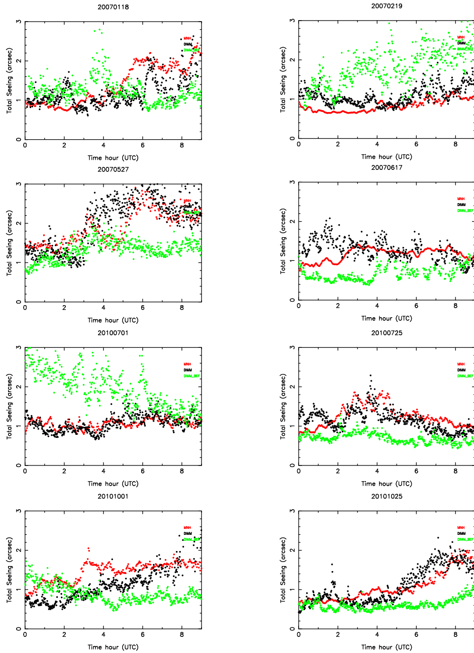
Figure 75: Temporal evolution of the total seeing as reconstructed by the model and observed by the DIMM (black line). The green line refers to the DIMM of the previous night.
