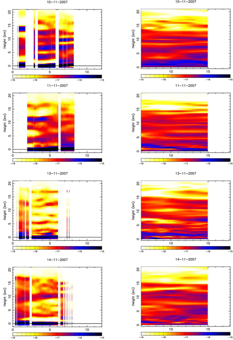
Figure 79: C_N^2 temporal evolution during the night. Left side: measurements provided by the Generalized SCIDAR. Right side: simulation provided by the model after the correction with the coefficient A_1 (see Section 5). The x-axis reports the time expressed in hours. For the image on the left side, these is time in UT therefore 00:00UT corresponds to 20:00 LT. For the image on the right side the hours correspond to the hours lasted from the beginning of the simulation (18:00UT of the day before). We have therefore that 06:00 corresponds to 20:00 LT. The two time cover therefore the same interval.
