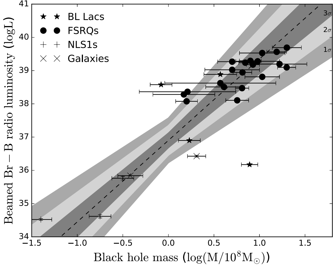
Figure 4. Observer-frame broad-band radio luminosity versus M_{\text{BH}} . The dashed line indicates the best-fit model. Symbols and grey areas as in Fig. 1.
