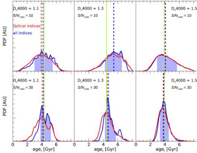
Fig. 13. Examples of PDFs of \text{age}_r of observed galaxies at z = 0.55 ; different values of D_n4000 = [1.1, 1.3, 1.5] (from left to right), and S/N_{l,\text{obs}} = 10 (upper panels) and S/N_{l,\text{obs}} = 30 (bottom panels) are shown. Probability density functions are retrieved using only optical indices (red distributions) and both ultraviolet and optical indices (blue distributions). The blue shaded region represents the confidence interval corresponding to the 16–84 per cent percentile range of the PDF. The solid green line corresponds to the true value of \text{age}_r = 4.31 Gyr, \text{age}_r = 4.44 Gyr, and \text{age}_r = 3.94 Gyr, respectively; the dashed vertical red (blue) line indicates the median value of the corresponding distribution.
