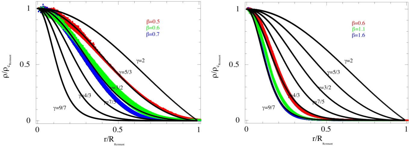
Fig. 8. Changes in the value of the polytropic index of the stellar remnant resulting from partial disruptions for selected initial values of its \beta . Densities and radii are normalised to the central density and the radius of the remnant. Black curves represent solutions to the Lane-Emden equation for different values of \gamma ; red, green, and blue points are from some of our simulations that left a remnant, for three different values of \beta . Left panel: \gamma = 5/3 polytrope. Right panel: \gamma = 4/3 polytrope.
